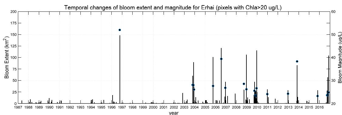
Figure 9. Temporal changes of bloom extent, defined as the area with Chl-a larger than 20 ug/L from 1987 to 2016. The bloom magnitude, which is the mean Chl-a for days with a bloom extent larger than 25 km 2 , are shown as dots.
