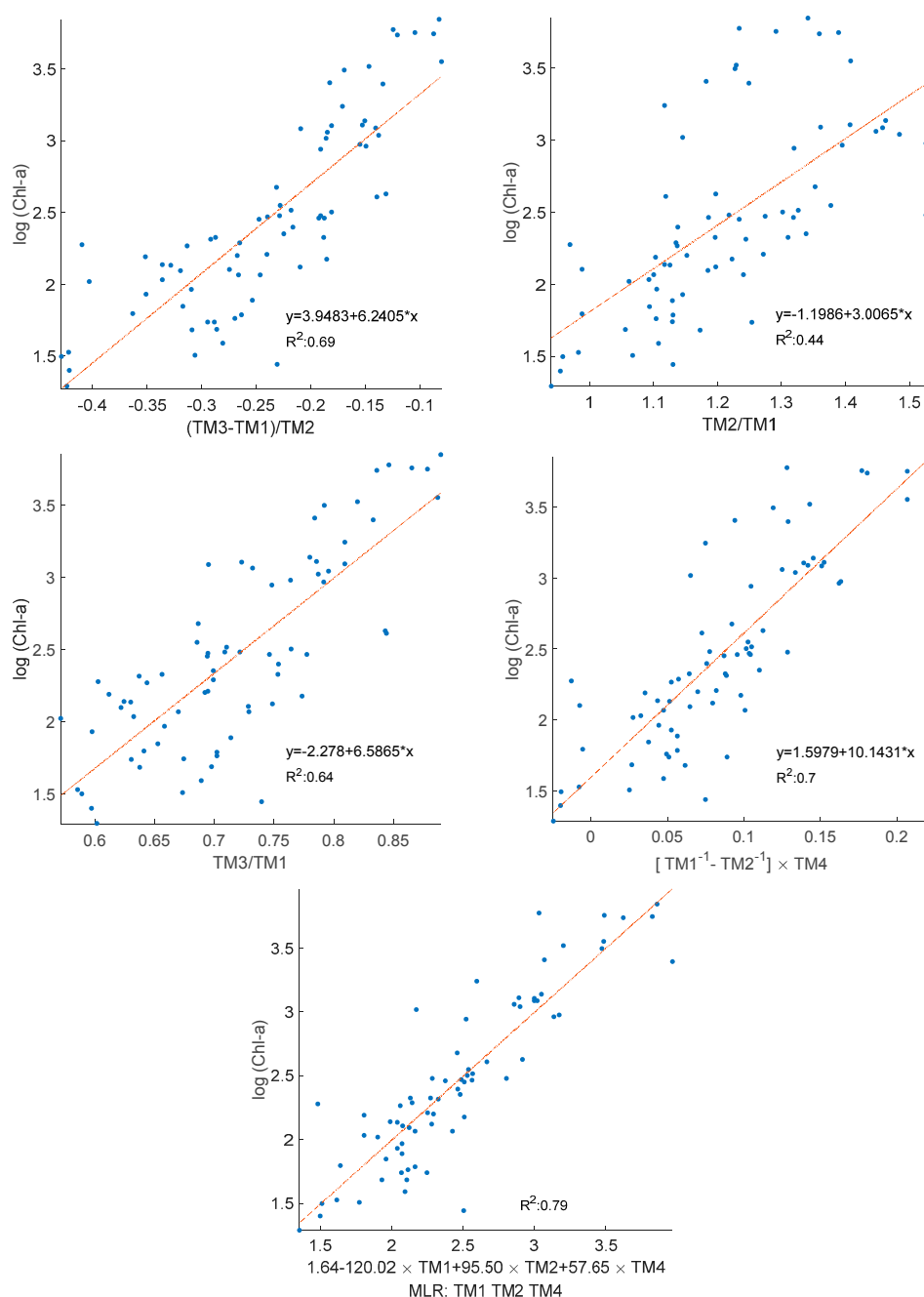
Figure 4. Comparison between estimated \log(\text{Chl-a}) and in situ \log(\text{Chl-a}) using different algorithms using in situ observations that have matched Landsat images within five days.
