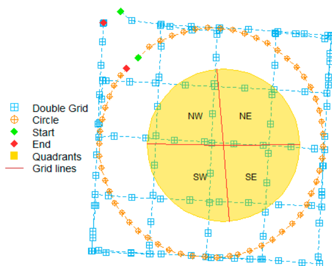
Figure 2. Generic Unmanned Aerial Vehicle data acquisition and flight pattern consisting of a double grid (blue) and a circular mission (orange). The two 15 m long grid lines (red) divide the plot area into four quadrants of similar size (yellow).
