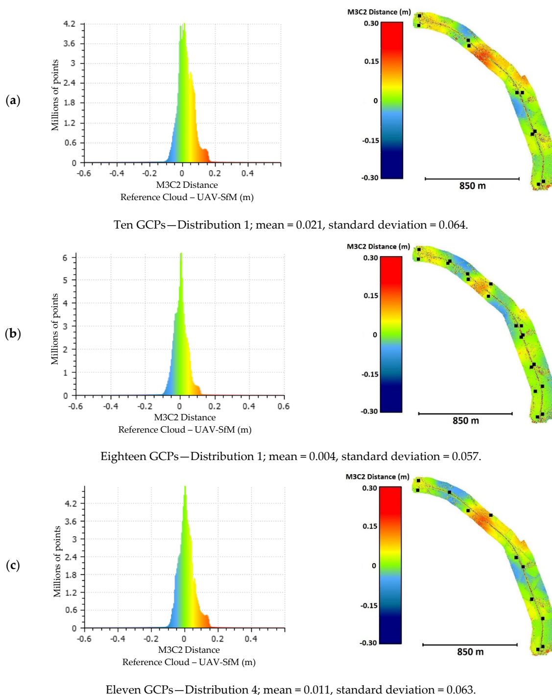
Figure 13. Distribution of errors for the M3C2-calculated distance between the reference cloud and the clouds obtained from the photogrammetric projects that used more than nine GCPs. The black squares represent the locations of the GCPs. (a) Project with 10 GCPs in Distribution 1, (b) project with 18 GCPs in Distribution 1, and (c) project with 11 GCPs in Distribution 4.
