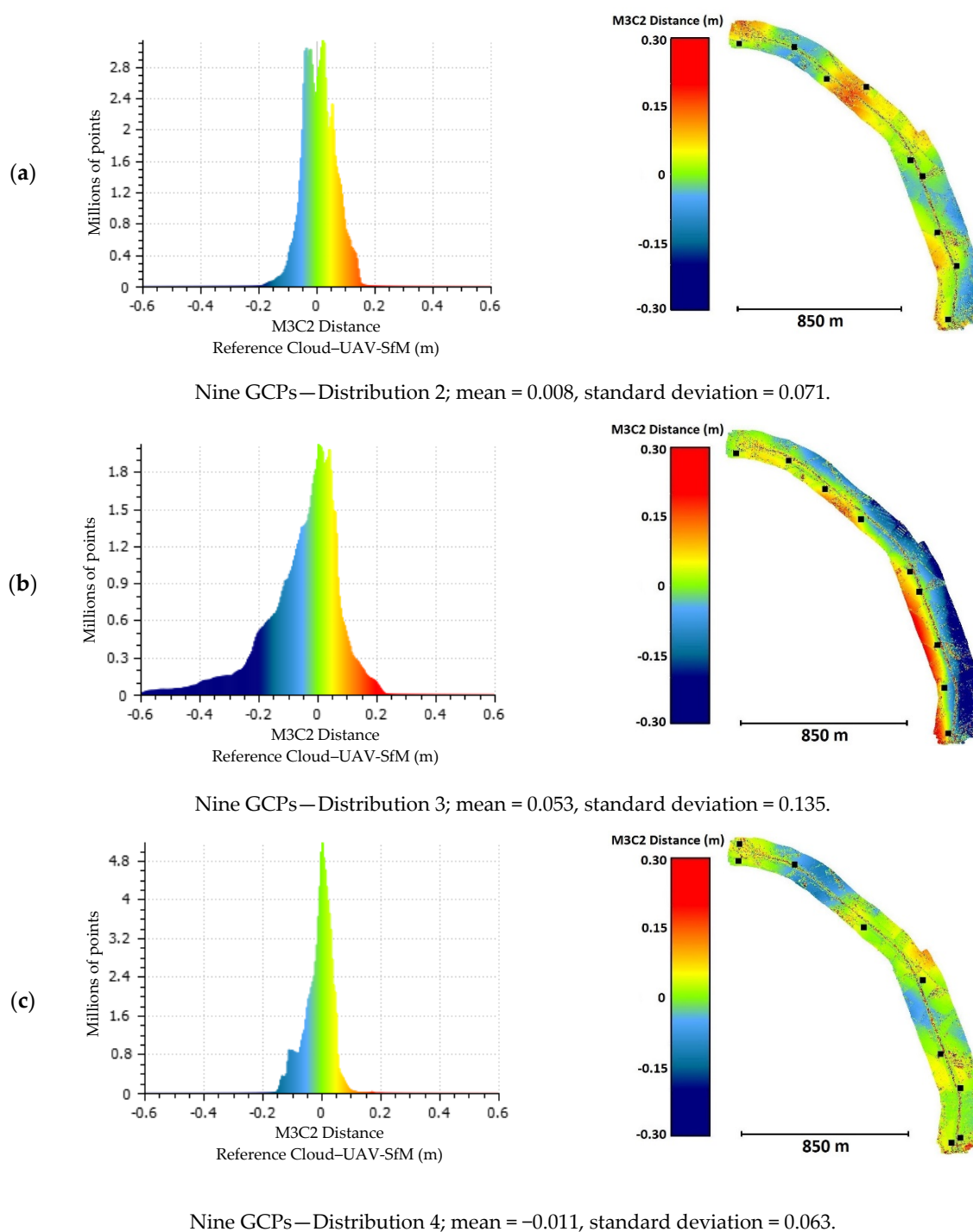
Figure 12. Distribution of errors for the M3C2-calculated distance between the reference cloud and the clouds obtained from the photogrammetric projects that used nine GCPs. The black squares represent the locations of the GCPs. (a) Distribution 2, (b) Distribution 3, and (c) Distribution 4.
