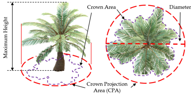
Figure 8. Illustration of height, crown area, and CPA.
