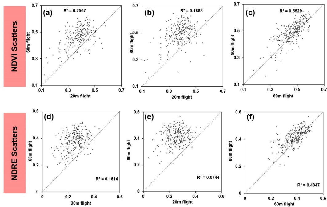
Figure 13. Scatterplot to compare NDVI and NDRE measured from different altitudes. Comparison between 20 m and 60 m (a) and (d), 20 m and 80 m (b) and (e), and 60 m and 80 m (c) and (f).
