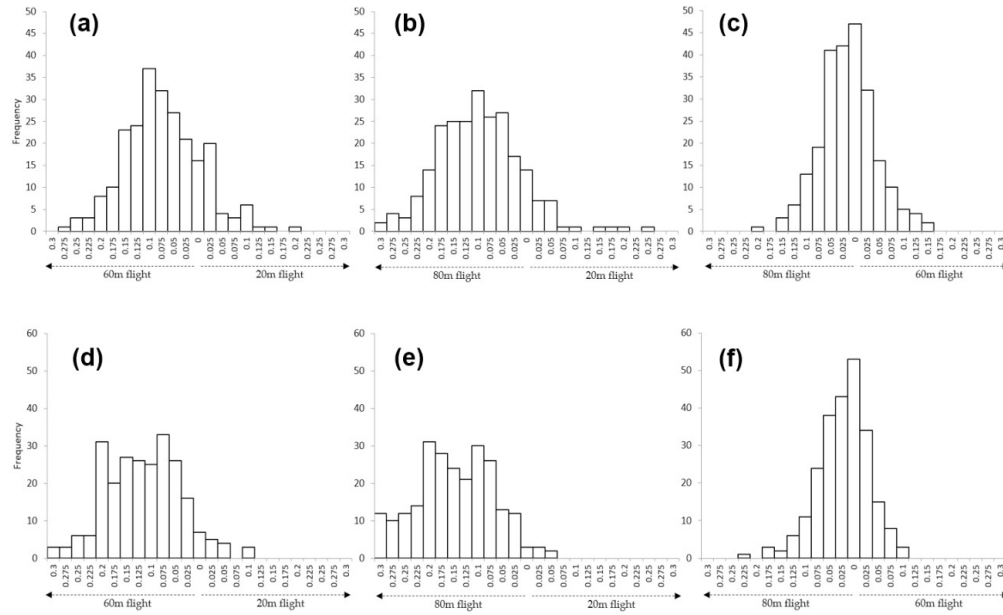
Figure 15. Histogram of difference for NDVI and NDRE between different flight altitudes: (a) and (d) between 60 m and 20 m, (b) and (e) between 80 m and 20 m, and (c) and (f) between 80 m and 60 m.
