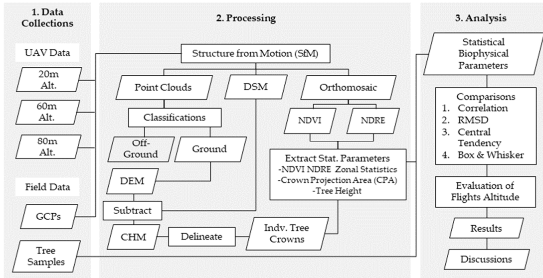
Figure 4. Flowchart of the methodology.
