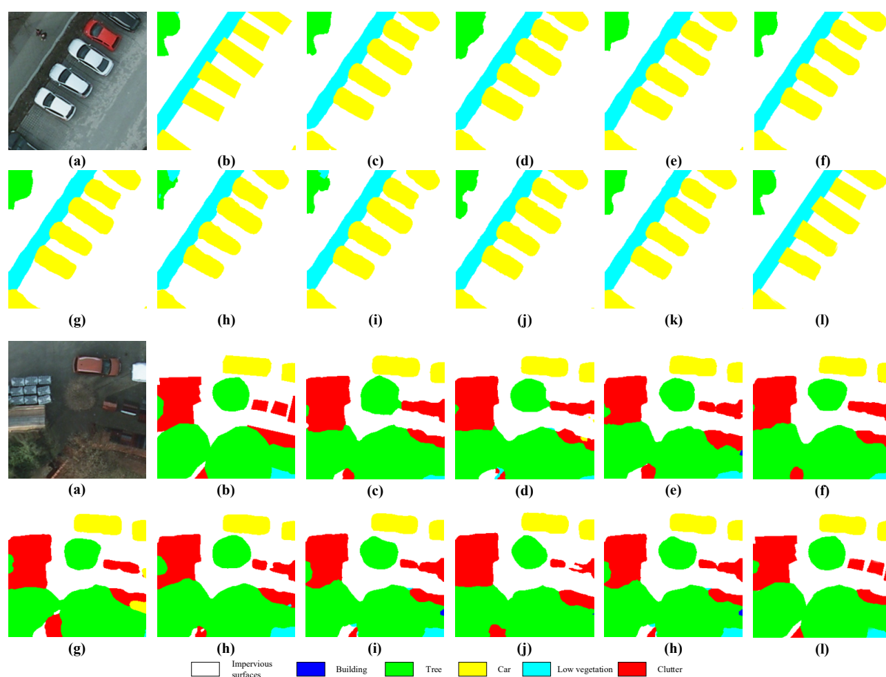
Figure 7. Visualization results on the Potsdam test set. (a) Original image, (b) Ground truth, (c) SegNet, (d) U-Net, (e) DeepLab V3+, (f) CBAM, (g) DANet, (h) OCNet, (i) NLNet, (j) ResUNet-a, (k) SCAttNet, (l) HCANet.
