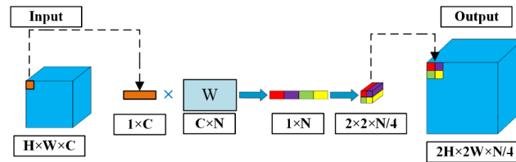
Figure 3. Pipeline of DUpSampling.
