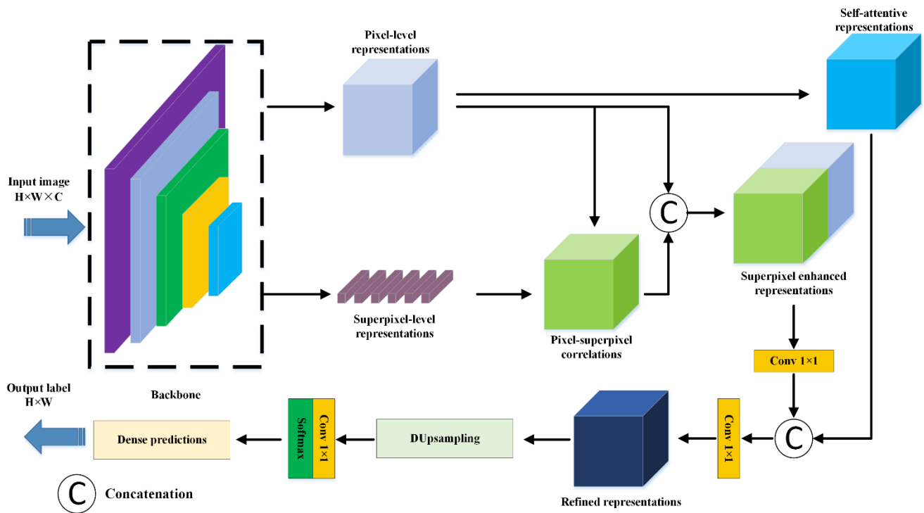
Figure 4. Overall framework of HCANet.
