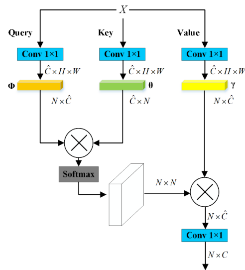
Figure 1. Non-local block.
