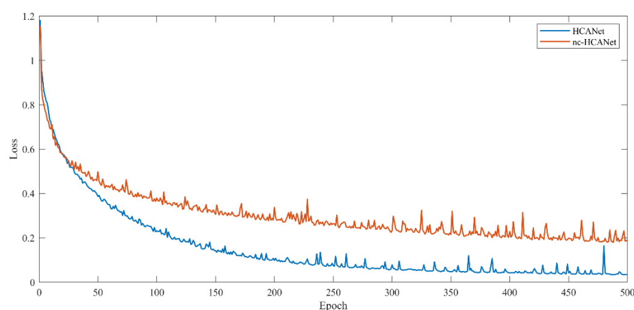
Figure 8. Training loss of Vaihingen dataset.
