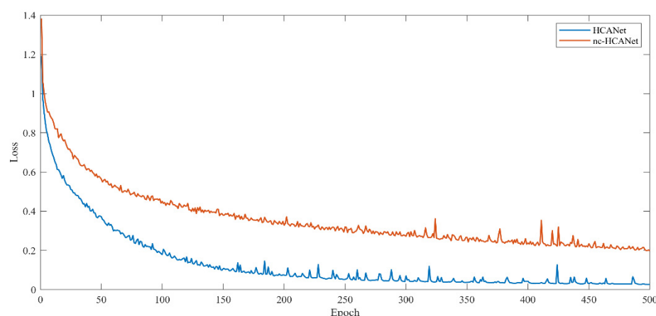
Figure 9. Training loss of Vaihingen dataset.
