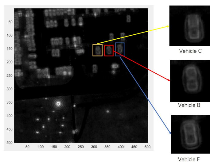
Figure 5. Full scene of entire 360° aperture after RPCA.
