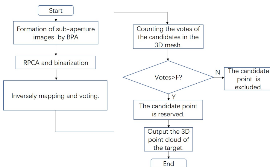
Figure 4. The algorithm flow chart of the proposed method.
