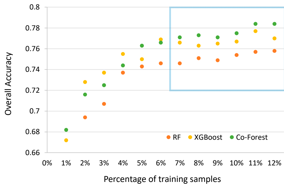
Figure 6. Comparison of the accuracy with traditional supervised algorithms at different levels of the training sample size.
