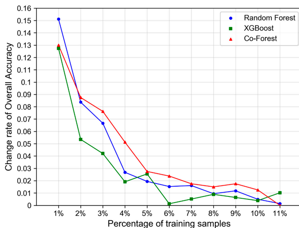
Figure 7. Change rate in classification accuracy at different training size ratios by taking the result with all training samples (12% in total) as a reference.
