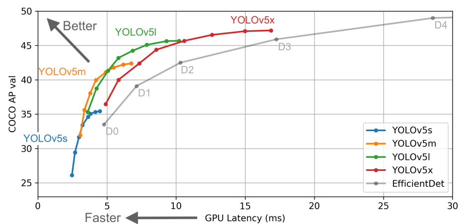
Figure 4. Performance comparison between YOLOv5 and EfficientDet [25]. COCO AP Val denotes the mAP metric measured on the COCO val2017 dataset over various inference sizes from 256 to 1536. The GPU speed measures the average inference time per image on the COCO val2017 dataset. It shows that the YOLOv5 family is much faster than EfficientDet with a good performance.
