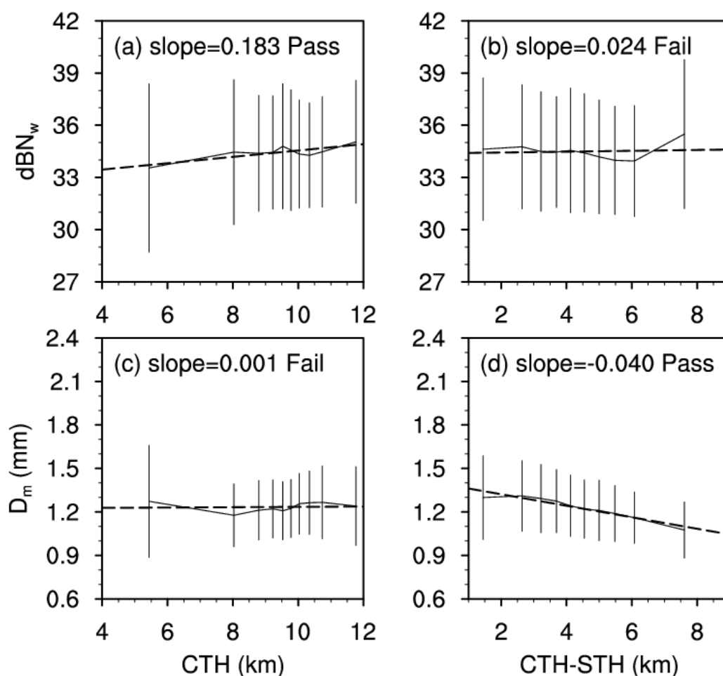
Figure 9. Relationship of (a,c) CTH and (b,d) CTH-STH with (a,b) dBN_w and (c,d) D_m for 2020-TC. Bars represent the standard deviation; the dashed line is the line of best fit for 10 equal-sample points; the panel lettering of each sub-figure is followed by the slope of the line of best fit and whether it passes the 95% significance test.
