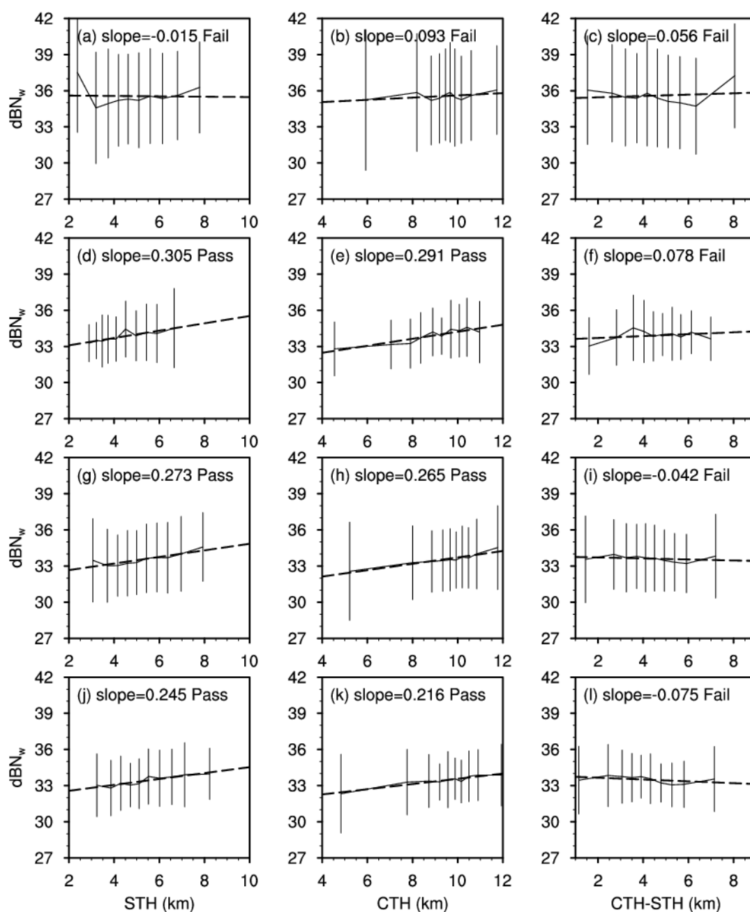
Figure 10. Relationship of STH (left), CTH (middle), and CTH-STH (right) with dBN_w during the 2020-TC period. According to the classification shown in Figure 8, the different dominant physical processes under the melting level are represented from top to bottom: (a–c) coalescence, (d–f) size-sorting or evaporation, (g–i) break-up, and (j–l) break-up and coalescence balance. Bars represent the standard deviation; the dashed line is the line of best fit for 10 equal-sample points; the panel lettering of each sub-figure is followed by the slope of the line of best fit and whether it passes the 95% significance test.
