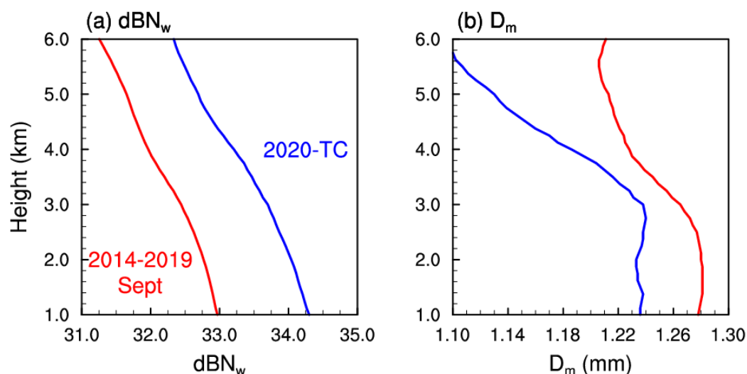
Figure 6. Vertical profiles for (a) dBN_w and (b) D_m . The blue line represents the 2020-TC period, and the red line represents the September 2014–September 2019 period.
