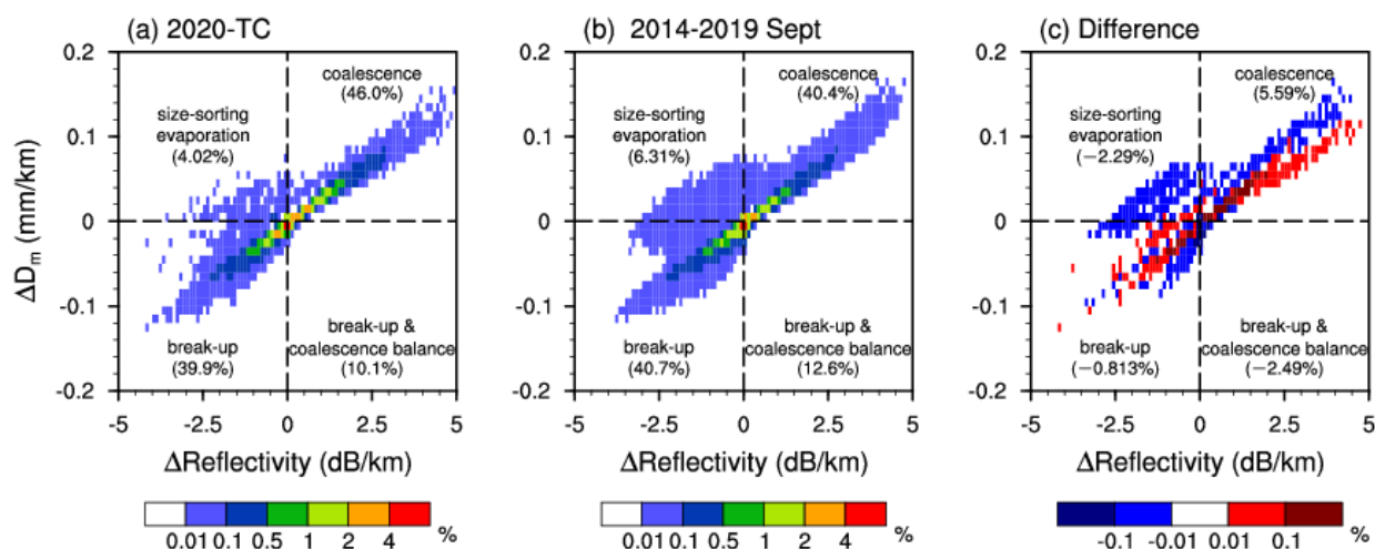
Figure 8. Frequency patterns in two-dimensional space of \Delta D_m and \Delta Reflectivity for (a) 2020-TC, (b) September 2014–September 2019, and (c) their difference (former minus the latter). The text in the figure represents the dominant microphysical processes and proportions in each quadrant.
