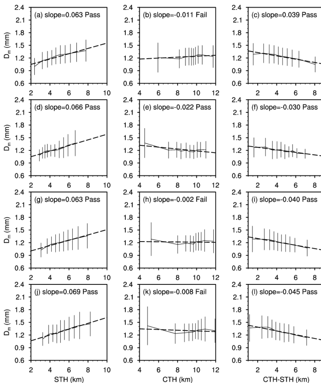
Figure 11. Relationship of STH (left), CTH (middle), and CTH-STH (right) with D_m during the 2020-TC pe-riod. According to the classification shown in Figure 8, the different dominant physical processes under the melting level are represented from top to bottom: (a–c) coalescence, (d–f) size-sorting or evaporation, (g–i) break-up, and (j–l) break-up and coalescence balance. Bars represent the standard deviation; the dashed line is the line of best fit for 10 equal-sample points; the panel let-tering of each sub-figure is followed by the slope of the line of best fit and whether it passes the 95% significance test.
