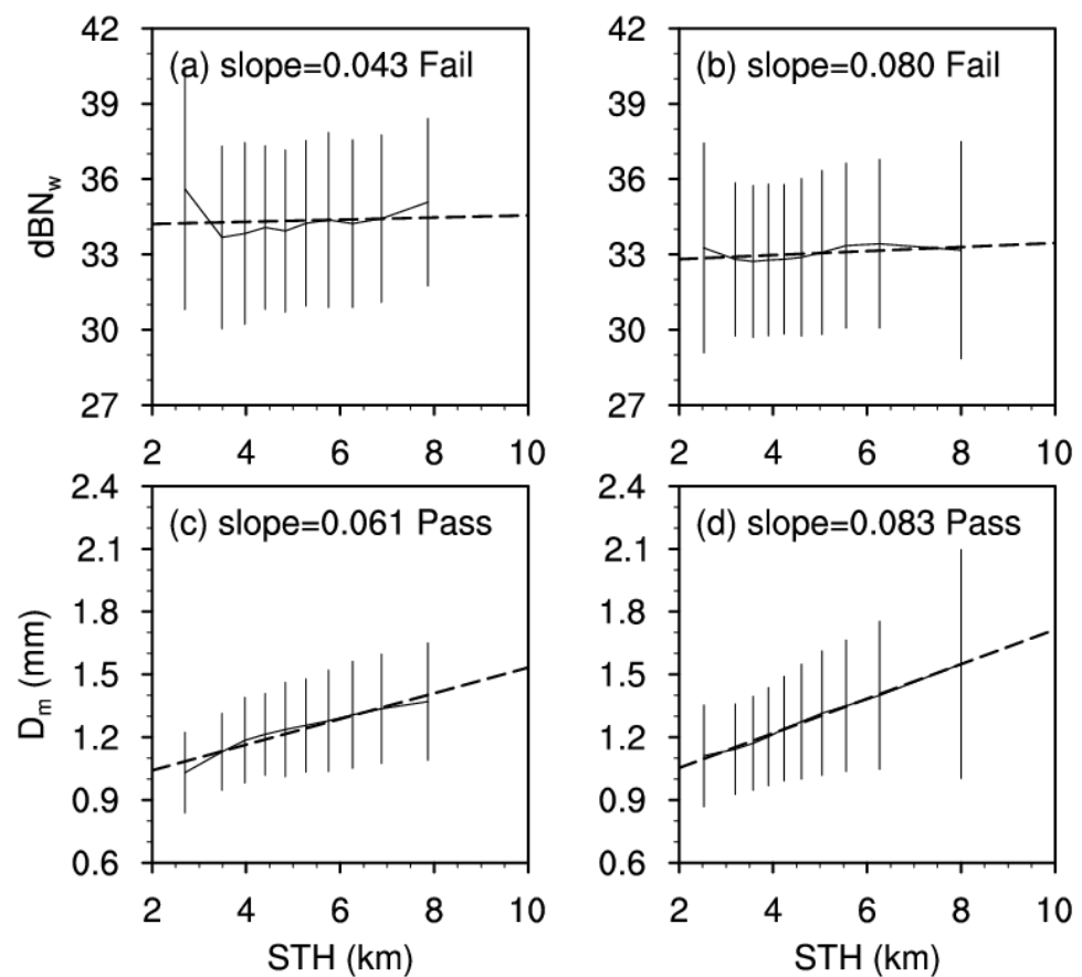
Figure 7. Relationship between STH and DSD: (a,b) STH vs. \text{dBW} ; (c,d) STH vs. D_m ; (a,c) 2020-TC; (b,d) September 2014–September 2019. Bars represent the standard deviation; the dashed line is the line of best fit for 10 equal-sample points; the panel lettering of each sub-figure is followed by the slope of the line of best fit and whether it passes the 95% significance test.
