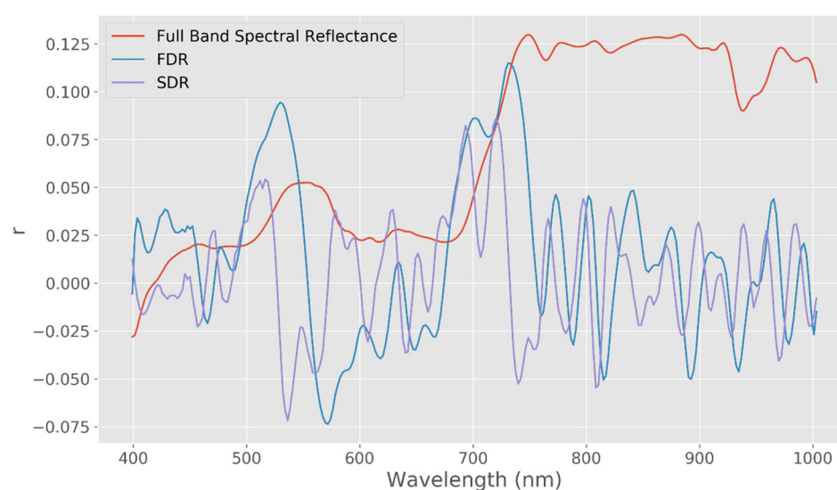
Figure 4. Pearson correlations between the spectral information and maize grain yield. The correlations were calculated for each spectral band at individual data collections. The averaged correlations over all the dates are shown in the plot.
