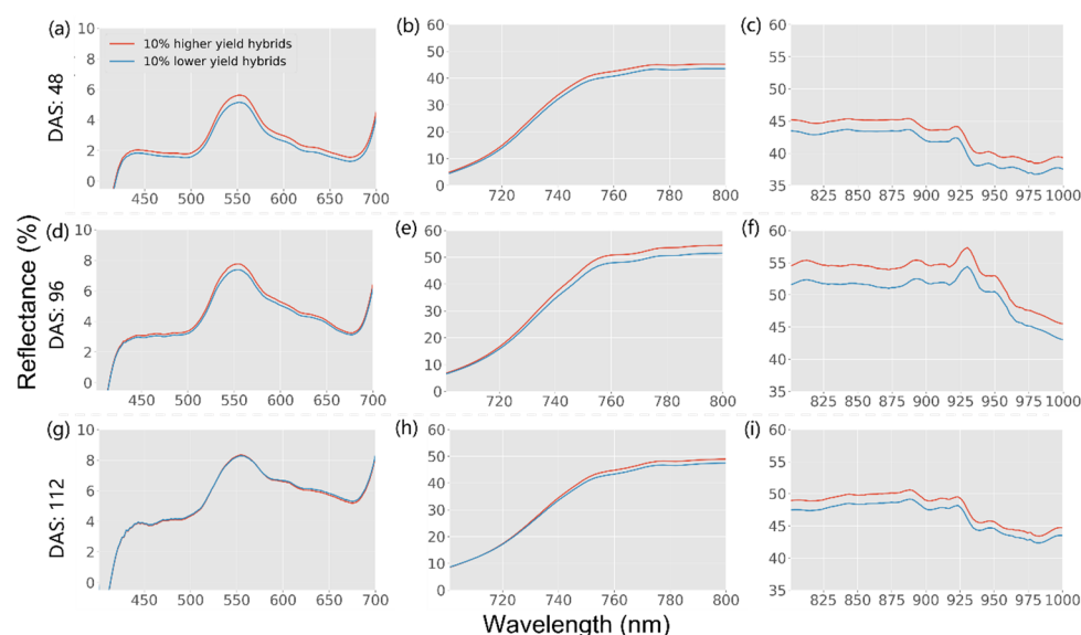
Figure 3. Spectral profiles of the hybrids with the top 10% and bottom 10% yields in the 400–700 nm (a,d,g), 700–800 nm (b,e,h), and 800–1000 nm (c,f,i) wavelength ranges at the early (a–c), middle (d–f), and late (g–i) growth stages.
