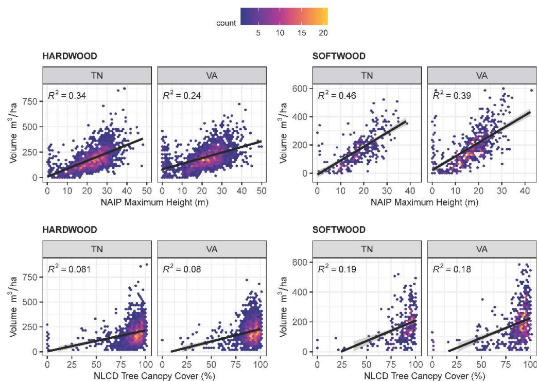
Figure 9. Scatter plots showing the relationship between NAIP maximum height (in meters, top row) and NLCD tree canopy cover (in %, bottom row) vs. FIA volume per area ( m^3/ha ) for hardwood (left column) and softwood (right column) species groups.
