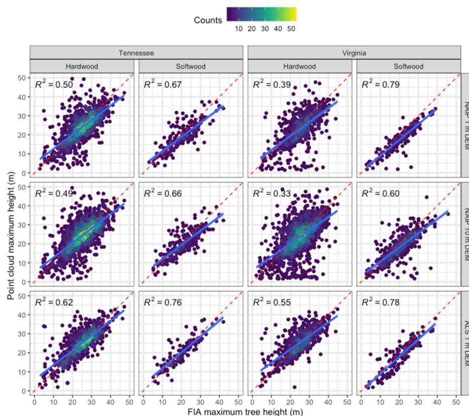
Figure 4. Scatter plot of FIA maximum tree heights (x-axis) vs. maximum point cloud heights (y-axis). Columns are broken out by state and species group (i.e., hardwood and softwood), while rows show the point cloud heights obtained for NAIP and ALS using different DEM resolutions. Plots are shaded from blue (low) to yellow (high) to indicate the density of observations that occur in places where multiple plots overlap. Blue lines are the reduced major axis regression (RMA) fits and the red dashed lines are the 1:1 lines.
