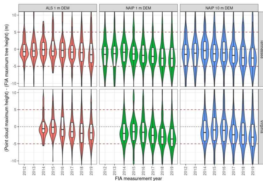
Figure 6. Differences between FIA maximum tree height and point cloud maximum height by FIA measurement year. Dashed red lines are drawn at \pm 5 m and dashed black lines at zero. For the boxplots, the bottom and top of the rectangles span the 25% to 75% height range, while the thick black bars are the median values. Columns break out the plots by point cloud source (ALS or NAIP) and DEM resolution (1 m and 10 m), while rows highlight the data collected in different states (TN top, VA bottom).
