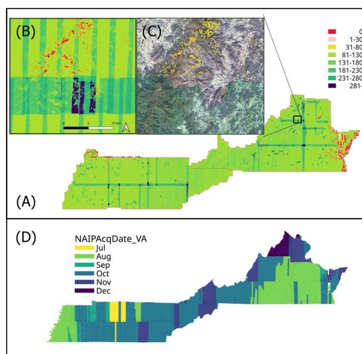
Figure 3. NAIP point cloud density and acquisition month. (A) Point density raster showing the number of 3D NAIP points in each 10-m grid cell. (B) A zoomed view of the point density raster. (C) A zoomed view of the NAIP imagery natural color composite. (D) NAIP imagery acquisition month.
