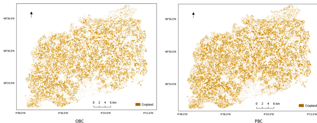
Figure 6. Level 2: PBC and OBC croplands extraction results.
