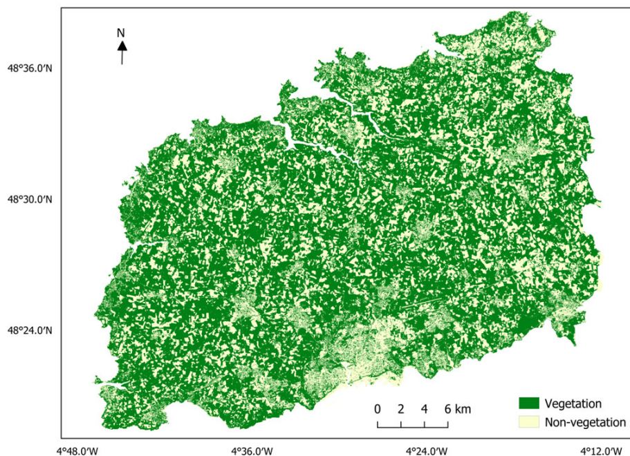
Figure 5. Level 1: PBC vegetation (including cropland) extraction results.
