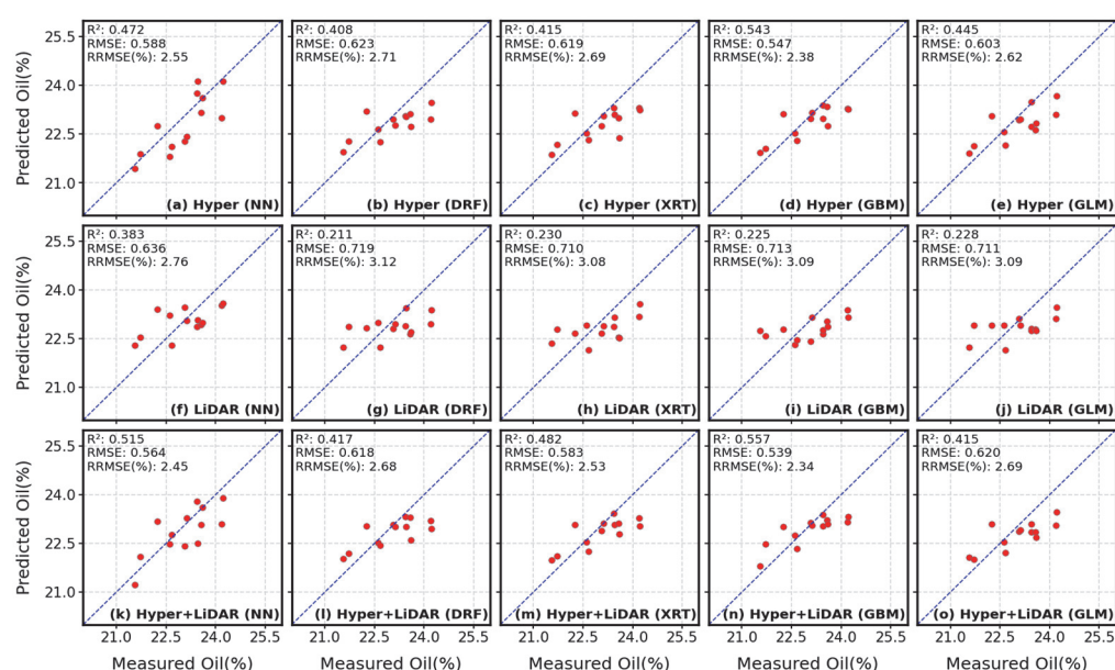
Figure 8. Scatter plots of measured vs. predicted soybean oil concentration using different models with hyper-based, LiDAR-based and Hyper + LiDAR-based features, respectively.
