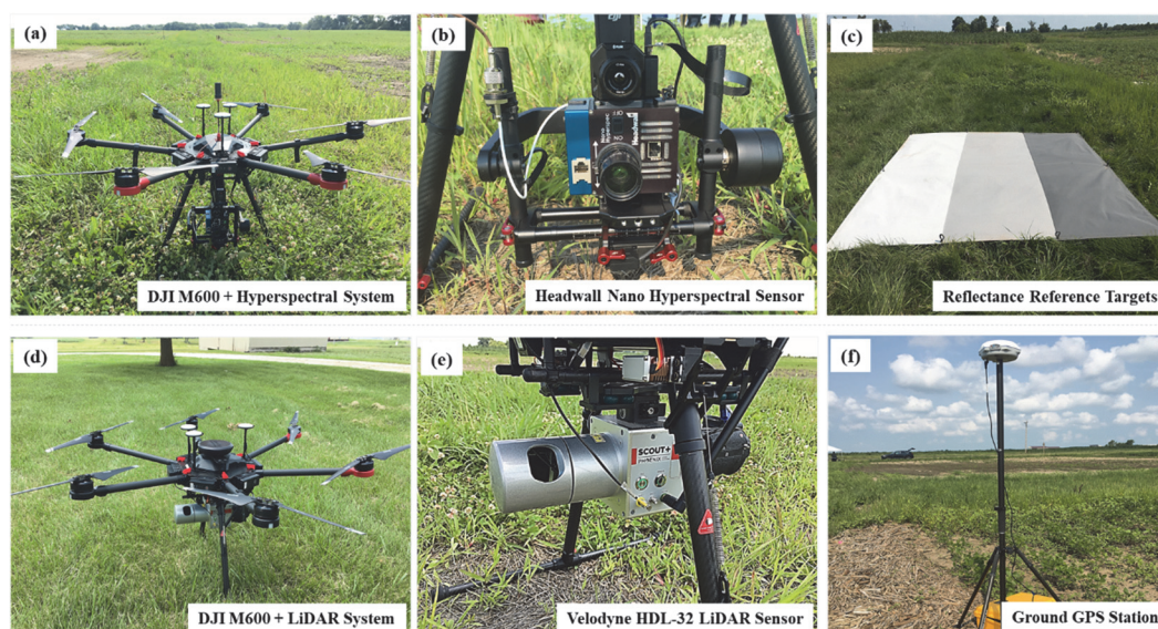
Figure 3. UAV systems and sensors used for data collection. (a) DJI M600 UAV platform with Hyperspectral Sensor. (b) Headwall Nano Hyperspectral Sensor. (c) Reflectance Reference Targets. (d) DJI M600 UAV platform with LiDAR sensor. (e) Velodyne HDL-32 LiDAR Sensor. (f) Ground RTK GPS Station. The figure was modified after [43].
