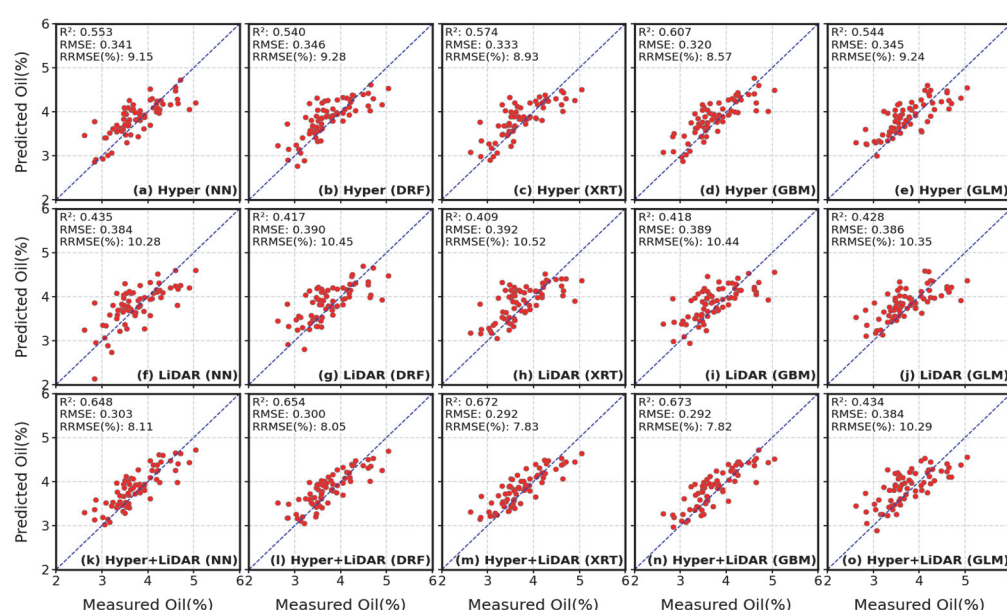
Figure 10. Scatter plots of measured vs. predicted corn oil concentration using different models with hyper-based, LiDAR-based and Hyper + LiDAR-based features, respectively.
