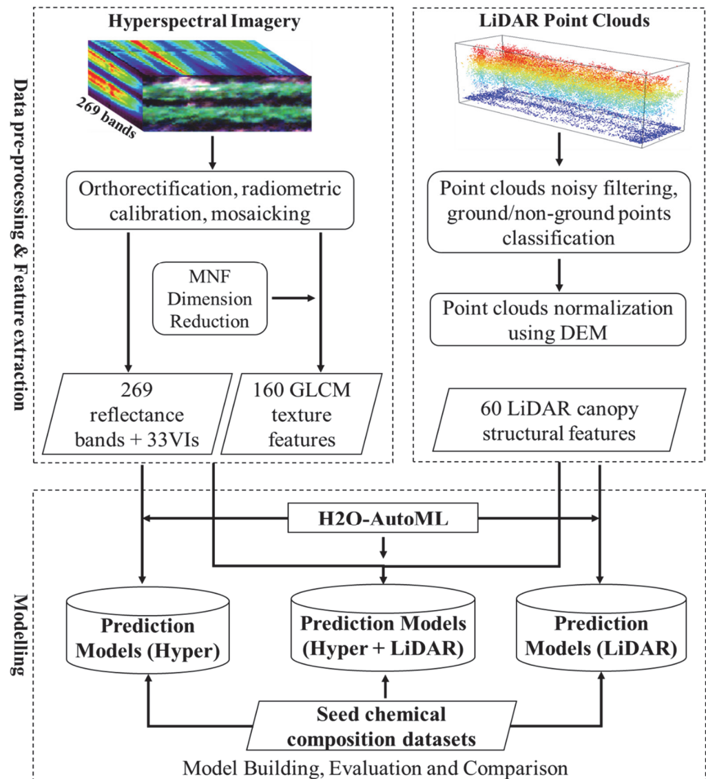
Figure 6. Workflow of hyperspectral and LiDAR data processing, feature extraction and implementing automated machine-learning methods. The figure modified after [43].
