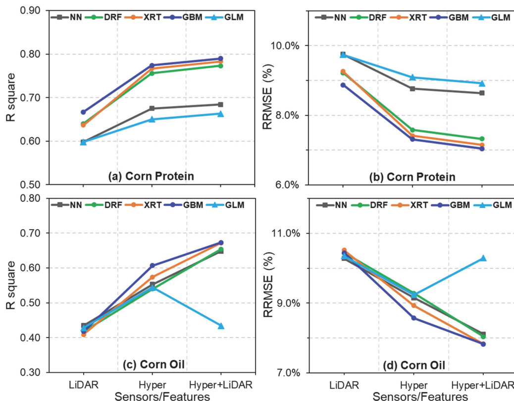
Figure 14. R^2 and RRMSE metrics when predicting corn protein and oil composition based on Hyperspectral, LiDAR and Hyper + LiDAR data using different machine-learning methods. ( R^2 : Coefficients of Determination, RRMSE: Relative Root Mean Square Error; NN: Deep Neural Network, DRF: Distributed Random Forest, XRT: Extremely Randomized Trees, GBM: Gradient Boosting Machine and GLM: Generalized Linear Model).
