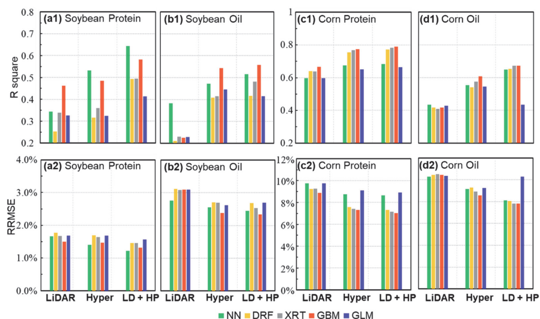
Figure 15. R^2 and RRMSE metrics when predicting soybean (a1,a2,b1,b2) and corn's (c1,c2,d1,d2) protein and oil composition based on Hyperspectral, LiDAR and LiDAR+Hyper (LD+HP) data using different machine-learning methods ( R^2 : Coefficients of Determination, RRMSE: Relative Root Mean Square Error; NN: Deep Neural Network, DRF: Distributed Random Forest, XRT: Extremely Randomized Trees, GBM: Gradient Boosting Machine and GLM: Generalized Linear Model).
