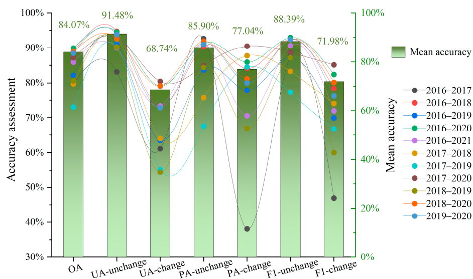
Figure 6. Validating the performance of the optimal threshold across eleven periods by utilizing the early winter wheat identification (EWWI) maps.
