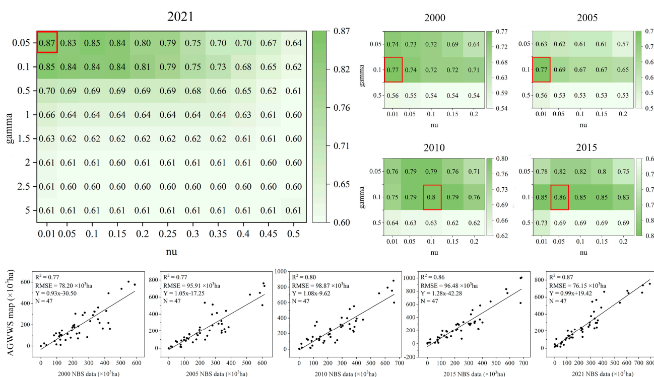
Figure 8. The significance ranking of R^2 under different parameter combinations and the correlation analysis between the winter wheat area depicted in AGWWS maps and the winter wheat area at the 47-city level from the National Bureau of Statistics.
