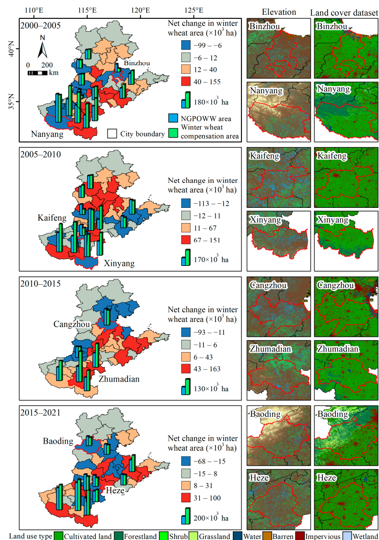
Figure 11. Distribution map of winter wheat net change areas by quantile and histograms of NGPOWW area and compensation area (1st column). Distribution of NGPOWW and compensatory planting areas for selected cities (2nd column), along with corresponding land use type distributions (3rd column).
