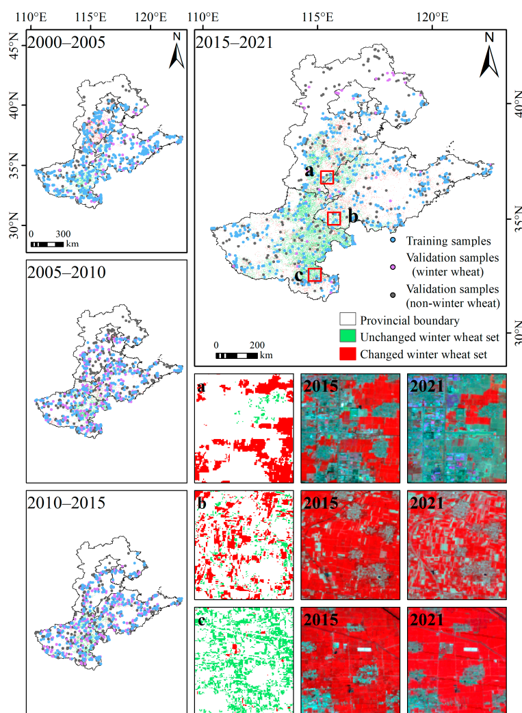
Figure 7. The spatial distribution of unchanged and changed winter wheat sample sets in each time period and the distribution of generated training and validation samples on the sample sets. (a–c)
