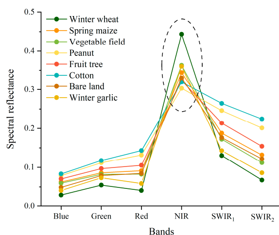
Figure 4. Average spectral reflectance of different crop pixels in Landsat images during the optimal phenological window. The dotted circle represents that the average NIR spectral reflectance of winter wheat is higher than that of other crops.
