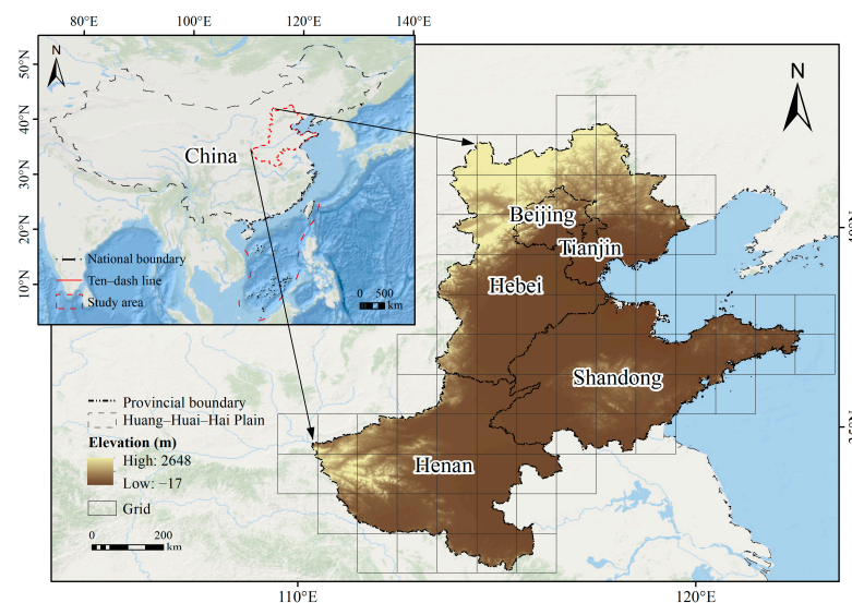
Figure 1. The study area and the grids covering the Huang–Huai–Hai Plain.
