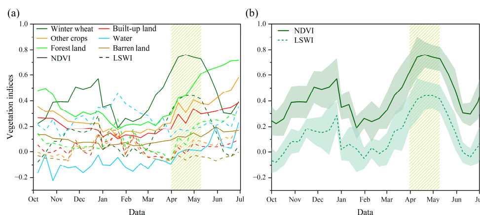
Figure 3. The ten-day average NDVI and LSWI time series for winter wheat and other land cover types (a) and the addition of the standard deviation range on the ten-day average time series of winter wheat, depicted in shaded areas (b). The dotted line represents the phenological window.
