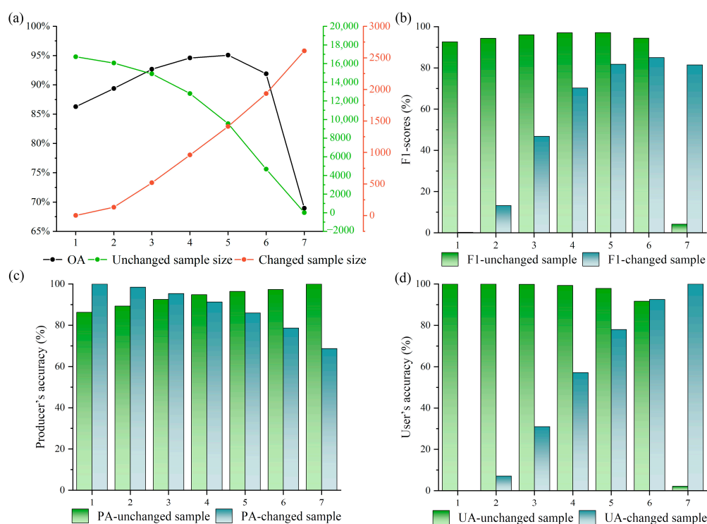
Figure 5. Variation of sample size and Overall Accuracy with different thresholds (a), F1 score (b), the Producer's Accuracy (c), and the User's Accuracy (d).
