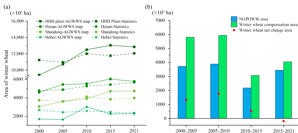
Figure 10. Winter wheat area changes over time in AGWWS maps and statistics (a). The Non-Grain Production of Winter Wheat (NGPOWW) area, winter wheat compensation area, and winter wheat net change area during each stage (b).
