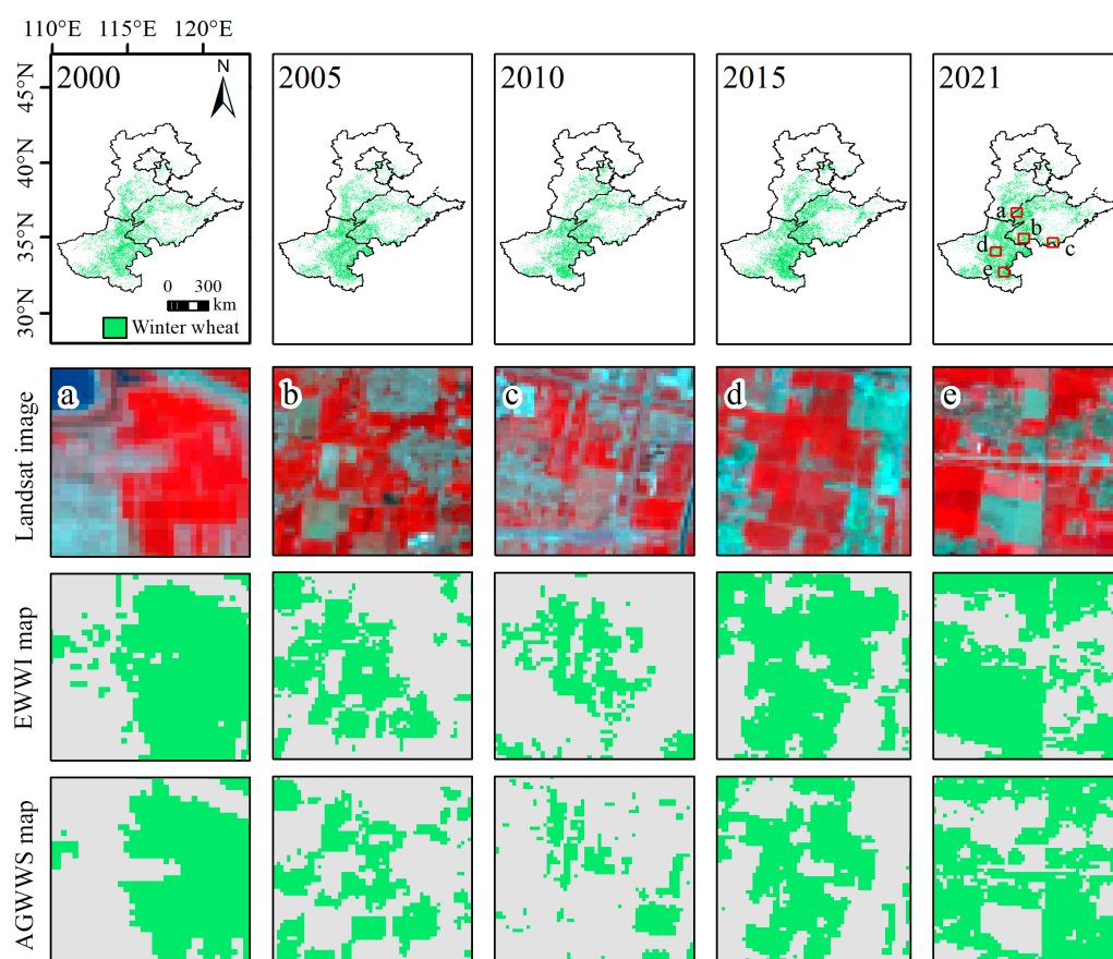
Figure 9. AGWWS maps for the study area in 2000, 2005, 2010, 2015, and 2021 (1st row). (a–e) represent the false-color composite of 2021 Landsat images at five different sites (2nd row), with EWWI maps and AGWWS maps at the corresponding sites (3rd and 4th rows).
