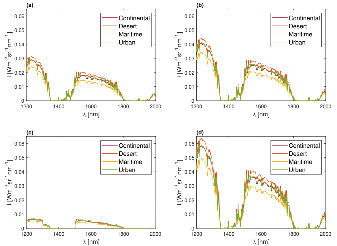
Figure 4. TOA radiance in 16 scenarios: variations in ‘Aerosol’ types and targeted ‘Surface’ at SZA of 20^\circ —(a) Pine forest, (b) Deciduous forest, (c) Ocean, and (d) Homogeneous snow.
