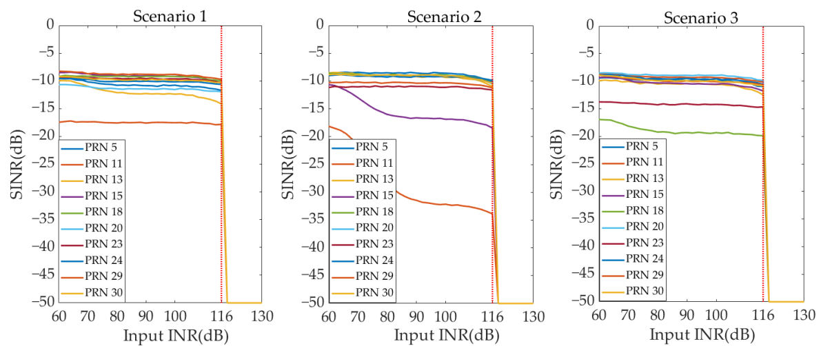
Figure 14. The SINR curve under different INR—hybrid beamforming (Scenarios 1–3).
