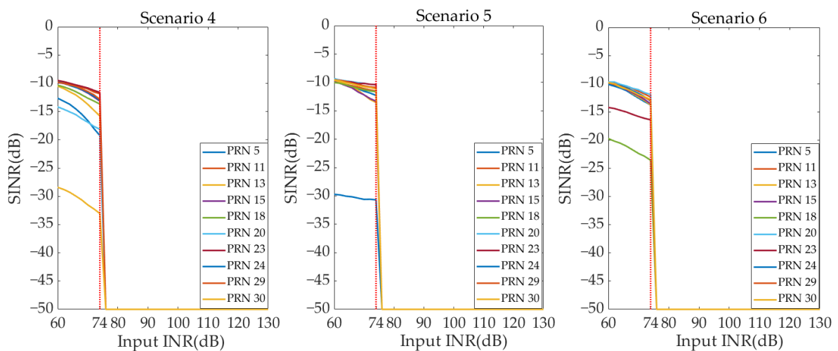
Figure 15. The SINR curve under different INR—digital beamforming (Scenarios 4–6).
