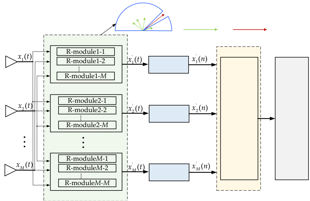
Figure 2. The hybrid array receiver structure.
