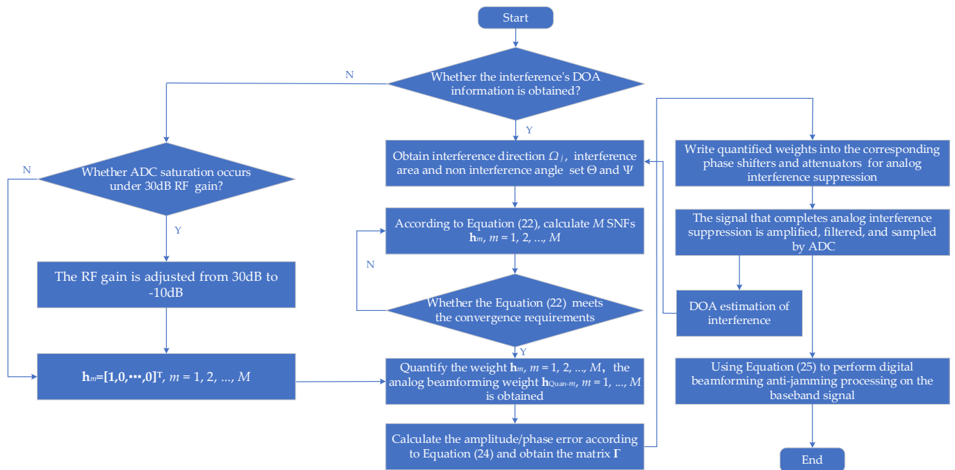
Figure 4. The flowchart of the proposed method.
