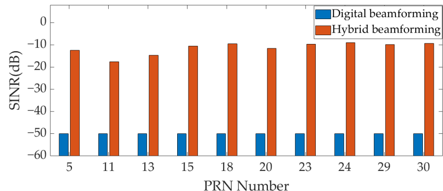
Figure 11. The output SINR under INR = 100 dB (Scenario 1).
