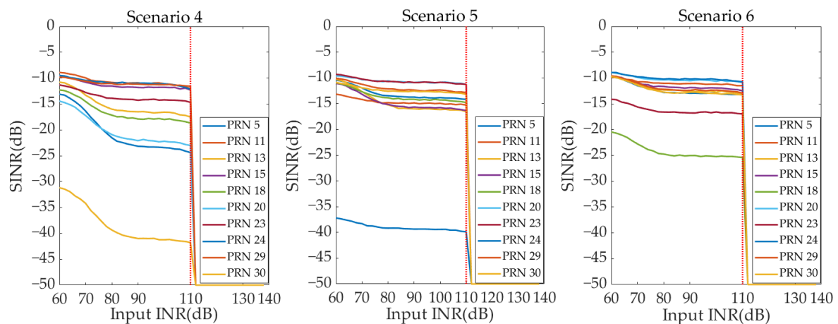
Figure 16. The SINR curve under different INR—hybrid beamforming (Scenarios 4–6).
