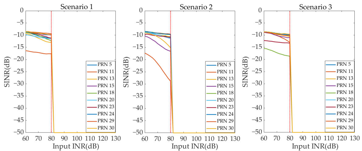
Figure 13. The SINR curve under different INR—digital beamforming (Scenarios 1–3).
