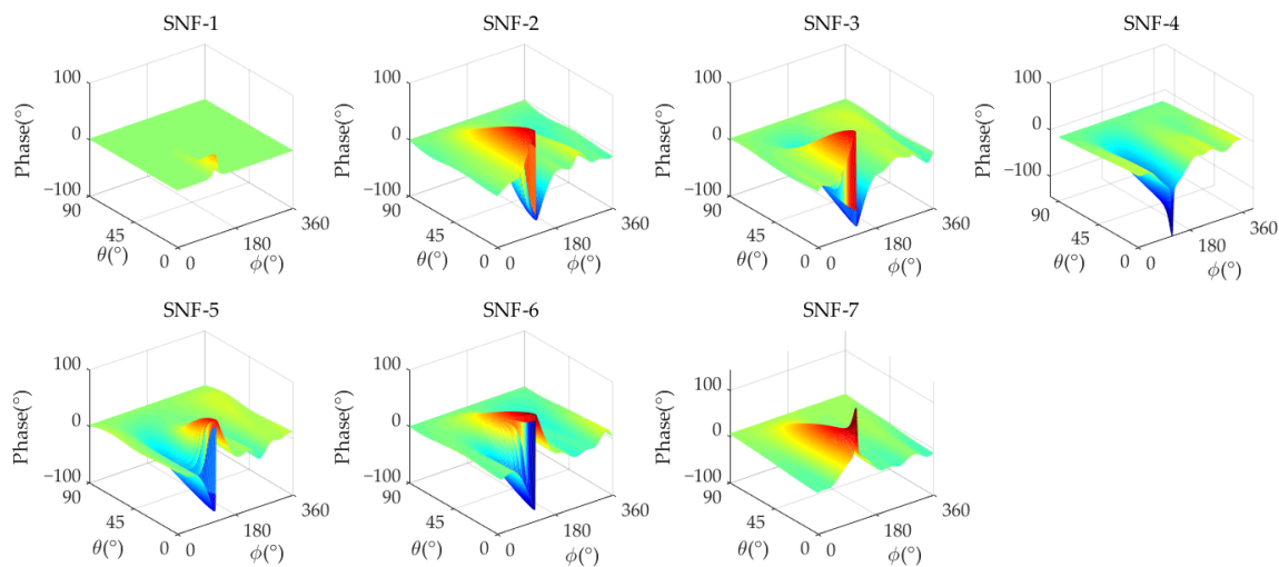
Figure 6. The analog MNF phase response of a 7-element antenna (Scenario 1).
