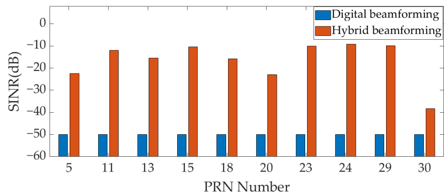
Figure 12. The output SINR under INR = 100 dB (Scenario 4).
