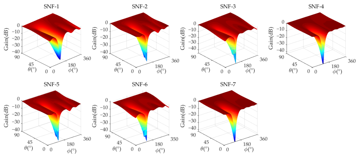
Figure 5. The analog MNF amplitude response of a 7-element antenna (Scenario 1).
