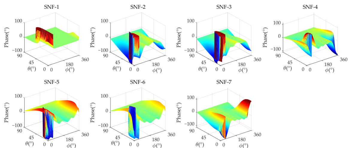
Figure 8. The analog MNF phase response of a 7-element antenna (Scenario 4).
