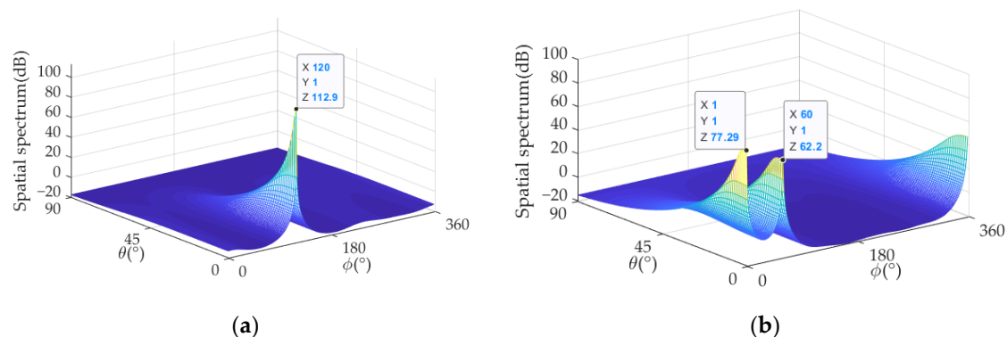
Figure 17. DOA estimation results under hybrid beamforming (INR = 100 dB). (a) DOA estimation result in Scenario 1. (b) DOA estimation result in Scenario 4.
