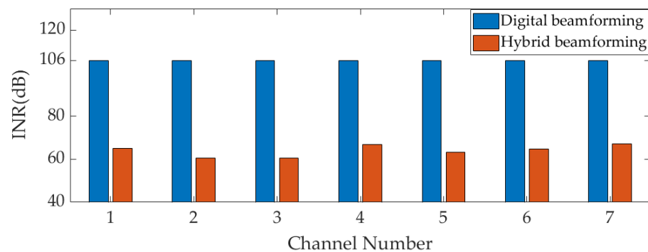
Figure 10. The INR of each RF channel before ADC sampling (Scenario 4).
