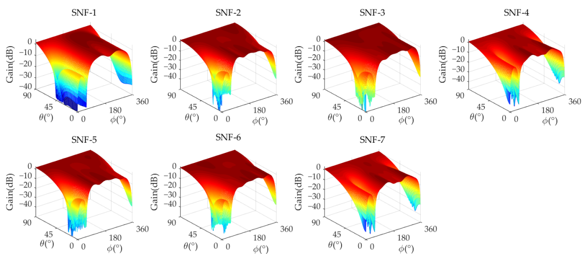
Figure 7. The analog MNF amplitude response of a 7-element antenna (Scenario 4).
