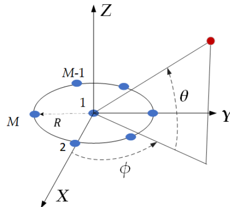
Figure 1. GNSS array antenna receiver configuration.
