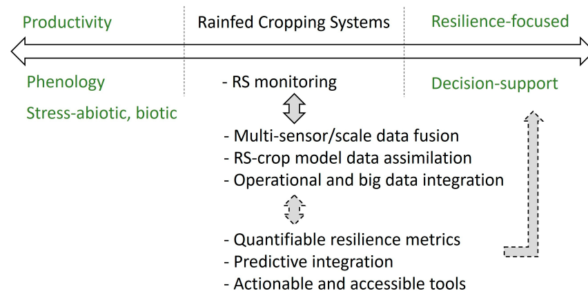
Figure 3. Conceptual pathway for transitioning remote sensing (RS) applications in rainfed cropping systems from productivity, phenology, and stress monitoring (left side, in green) toward resilience-focused and decision-support outcomes (right side, in green). Note: Double-headed arrows represent interactive feedback loops; Black solid arrows indicate the emerging approaches along this pathway; Dashed arrows and lines denote the proposed directions toward resilience.
