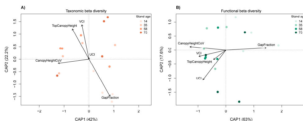
Figure 3. Distance-based redundancy analysis (dbRDA) ordinations of taxonomic beta diversity (orange; (A)) and functional beta diversity (green; (B)) of understory plant communities constrained by forest structural metrics. Points represent 13-m-radius plots and are coloured according to successional stage. Plots located closer together in the ordination space have more similar community composition than plots located farther apart. Arrows represent forest structural variables; arrow direction indicates the direction of increasing values of the corresponding variable, whereas arrow length is proportional to the strength of its association with the ordination axes. Analyses were conditioned on chronosequence. The percentages reported in parentheses on the CAP1 and CAP2 axes indicate the proportion of constrained variance explained by each canonical axis.
