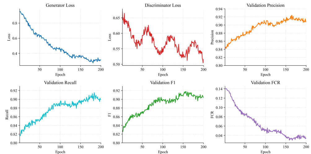
Figure 5. Training stability analysis of Attention-GAN. The curves show the generator loss, discriminator loss, validation precision, validation recall, validation F1, and validation FCR over 200 epochs.
