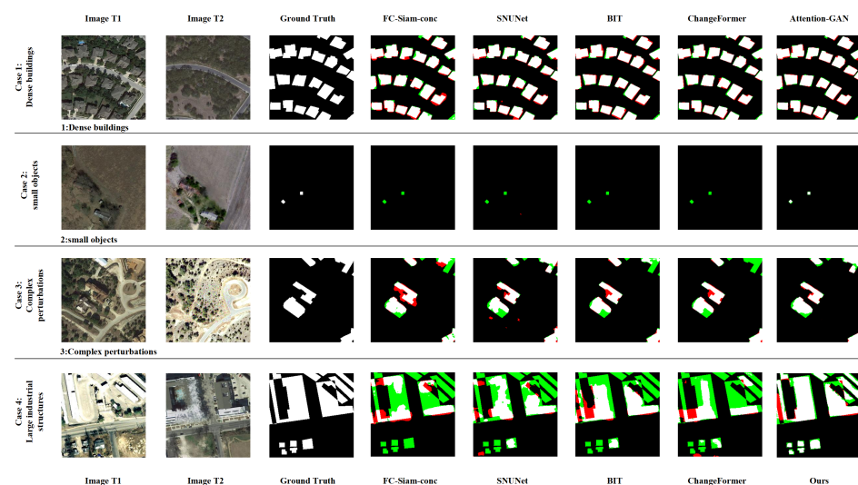
Figure 2. Representative visual results for four test scenes. Columns show the bi-temporal images, ground truth, selected baseline predictions, and the proposed Attention-GAN prediction. In the prediction overlays, white pixels indicate correctly detected changed pixels, green pixels indicate omission errors, and red pixels indicate false alarms.
