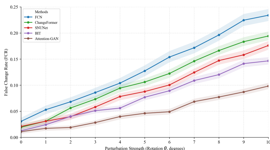
Figure 3. Robustness degradation curve under rotation perturbation. FCR vs. \theta \in [0, 10^\circ] ; shaded region shows standard deviation over three runs. FCN denotes the fully convolutional early-fusion baseline used in this robustness comparison.
