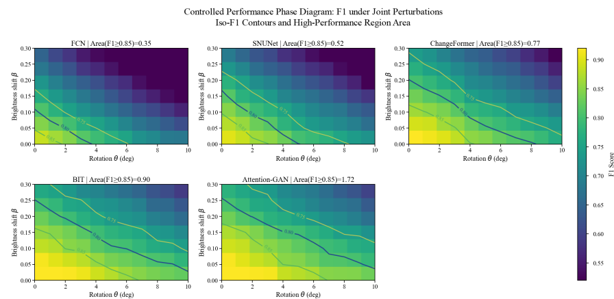
Figure 4. Controlled 2D performance phase diagram under joint rotation ( \theta ) and brightness ( \beta ) perturbations. Color indicates F1 score on perturbed held-out test pairs with valid reference change masks; contours show F1 \geq 0.85 region. FCN denotes the fully convolutional early-fusion baseline used in this robustness comparison.
