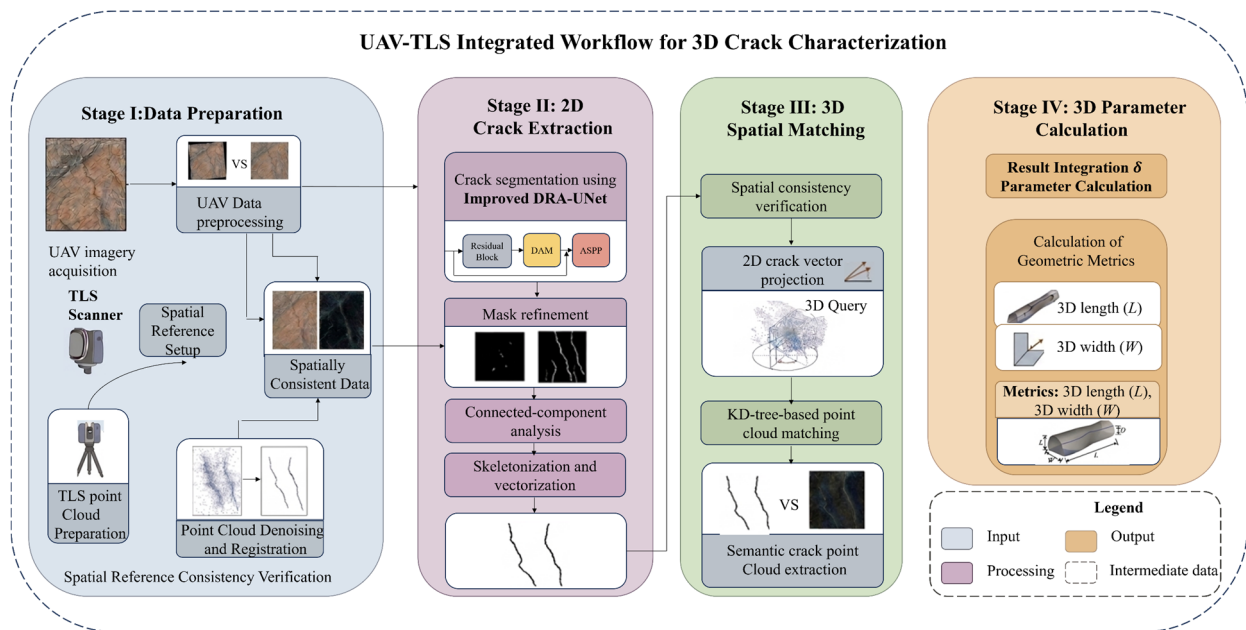
Figure 2. Overall workflow of the UAV–TLS fusion framework for mining-induced surface crack extraction, 3D spatial mapping, and geometric parameter estimation. The arrows indicate the processing sequence, and the different colors distinguish the main workflow stages and data-processing modules.
