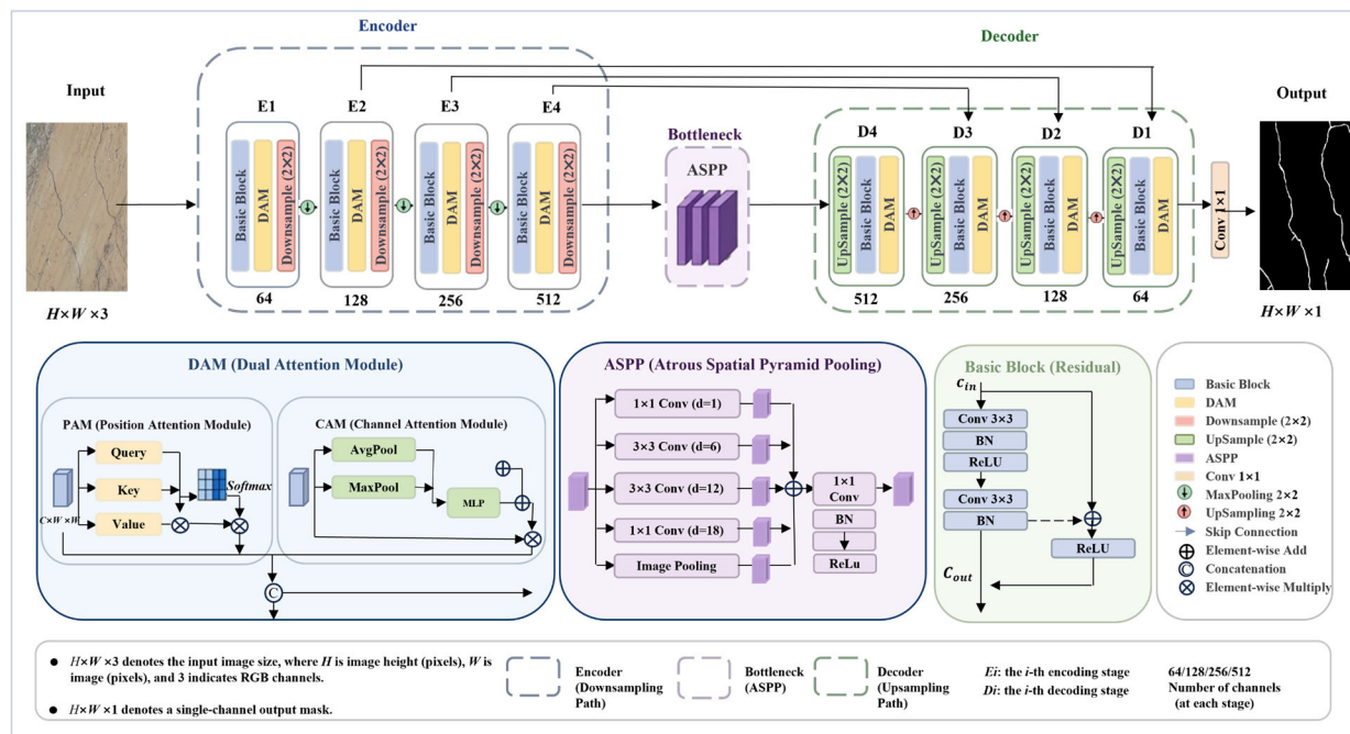
Figure 3. Architecture of DRA-UNet and its key components for mining-induced surface crack segmentation. The ASPP output serves as the primary input to the decoder, while encoder skip features provide auxiliary high-resolution information. At each decoder stage, the upsampled decoder feature map is fused with the corresponding encoder feature map at the same spatial resolution by channel-wise concatenation followed by convolutional refinement.
