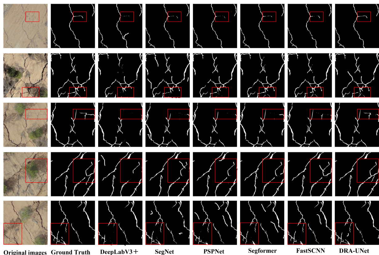
Figure 5. Visual comparison of crack semantic segmentation results obtained by different deep learning models. The red boxes highlight representative local regions used to compare crack extraction details among different models.
