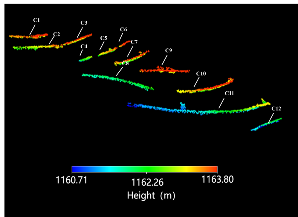
Figure 7. 3D semantic crack point clouds of representative cracks and their corresponding labels.
