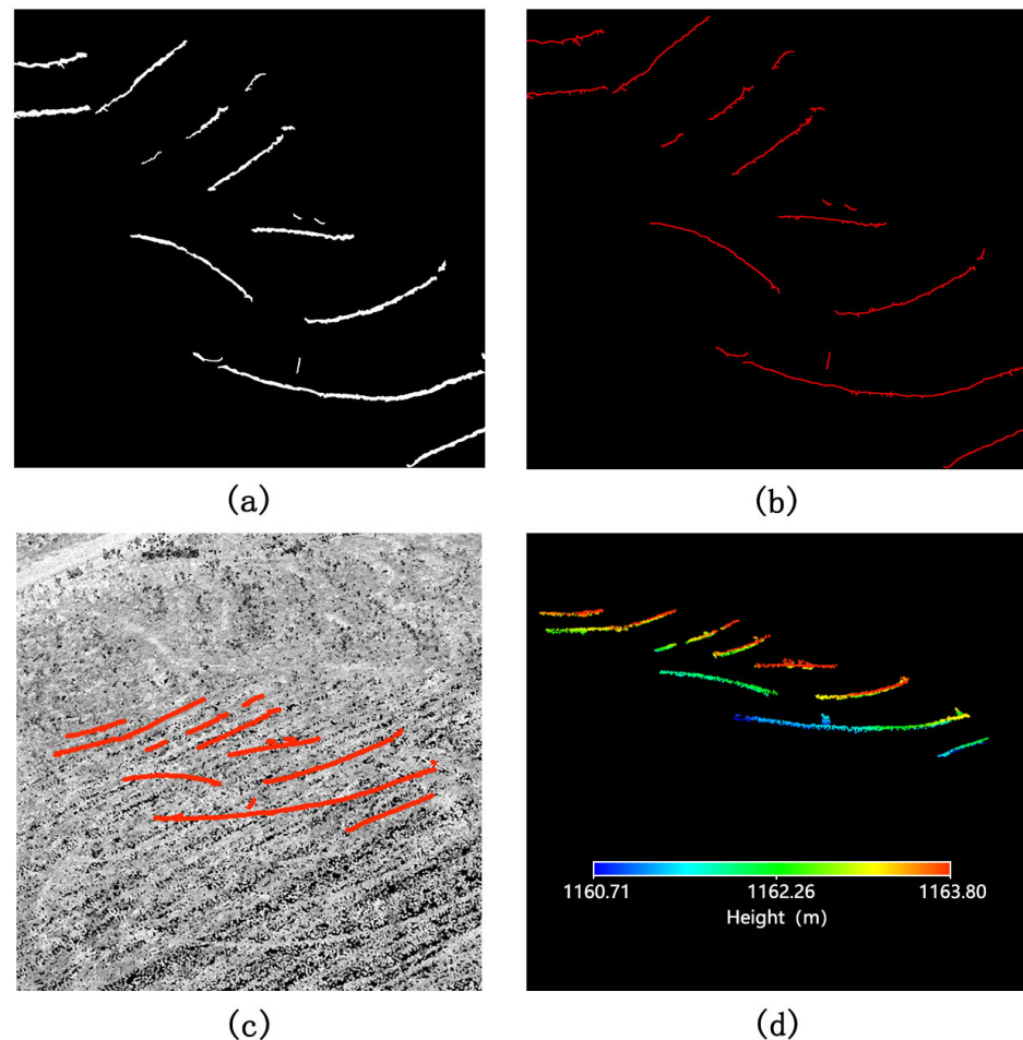
Figure 6. Results of crack extraction and 3D spatial mapping. (a) Binarized crack segmentation; (b) extracted crack skeleton; (c) mapping of crack skeleton onto TLS point cloud; (d) semantic crack point cloud after KDTree spatial matching. The colors in the point cloud indicate elevation variations, and the red lines/points represent crack-related features.
