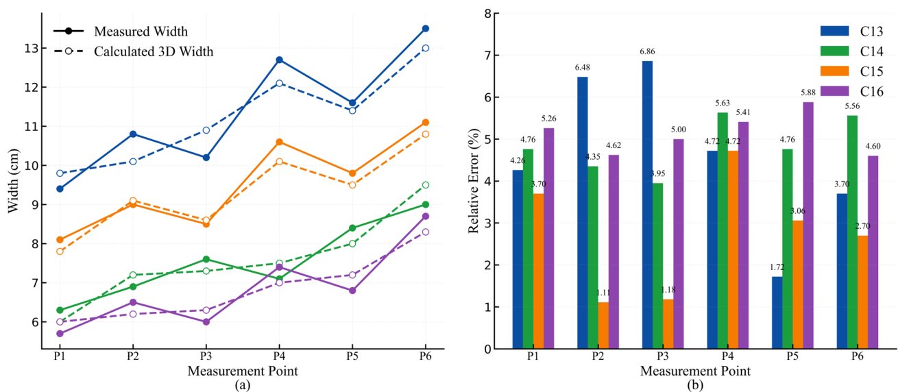
Figure 9. Validation of calculated 3D crack width results. (a) Comparison between field-measured widths and calculated 3D widths; (b) analysis of relative errors. Different colors represent different representative cracks used for width validation.
