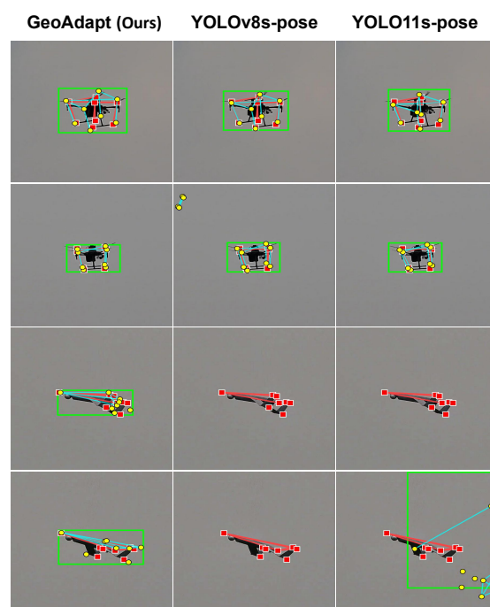
Figure 5. Zero-shot keypoint detection on real long-range optical images. Green denotes the predicted bounding box; cyan and yellow denote the predicted eight-keypoint configuration; and red squares and lines denote the manually annotated ground truth. Rows 1–2 show the Matrice 200 quadrotor, and Rows 3–4 show the fixed-wing ScanEagle.
