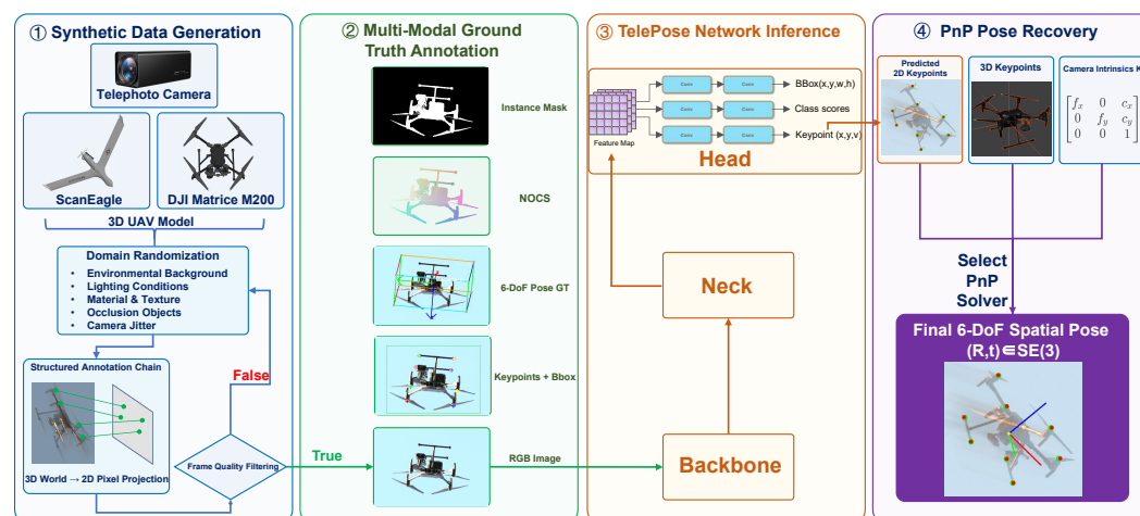
Figure 1. End-to-end GeoAdapt pipeline comprising synthetic-data generation with domain randomization, multimodal ground-truth anchoring, deformable keypoint detection, and Perspective- n -Point (PnP)-based six-degree-of-freedom (6-DoF) pose recovery for ground-based optical remote sensing. UAV, unmanned aerial vehicle; 2D, two-dimensional; 3D, three-dimensional; RGB, red–green–blue; GT, ground truth; Bbox, bounding box; NOCS, normalized object coordinate space; Conv, convolution; and SE(3), special Euclidean group in three dimensions.
