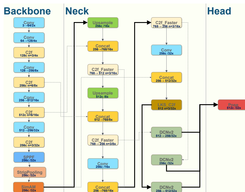
Figure 2. GeoAdapt network architecture. The model comprises a C2f backbone with a triple-enhanced P5 stage, a hybrid C2f_Faster + LKS_C2f neck, and deformable convolution v2 (DCNv2) feature-refinement modules inserted between the neck and the standard pose head at each feature pyramid network (FPN) scale.
