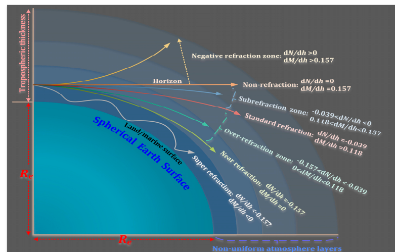
Figure 2. Different tropospheric atmospheric refraction types. The propagation path of EM waves in the troposphere is primarily determined by either dM/dh or dN/dh , enabling the classification of atmospheric refraction characteristics based on these parameters. When dM/dh < 0 or dN/dh < -0.157 N-units/m, EM wave rays bend towards the Earth's surface, becoming trapped within a thin atmospheric layer.
