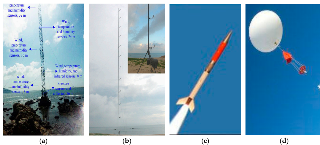
Figure 4. Several atmospheric duct detection instruments: (a) meteorological tower [343], (b) gradiometer [176], (c) rocketsonde, and (d) airship.
