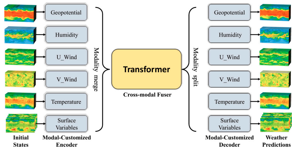
Figure 16. Overview of FengWu LWM [418].
