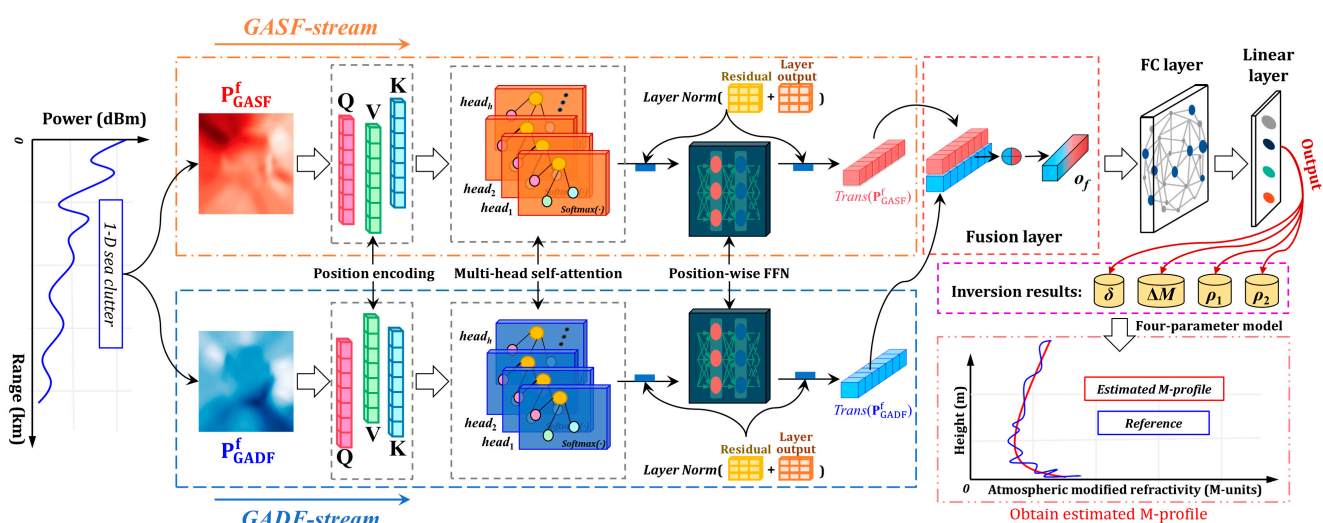
Figure 14. RFCFormer [190]. This model takes 1D radar sea clutter as input and transforms it into two spatially distributed 2D matrices ( P_{GASF}^f and P_{GADF}^f ) using GAF-based Gramian Angular Sum Field (GASF) and Gramian Angular Difference Field (GADF). These matrices are processed through a dual-stream Transformer architecture, where positional encoding, multi-head attention mechanisms, and feedforward neural network (FFN) extract hierarchical features, followed by feature fusion in a
