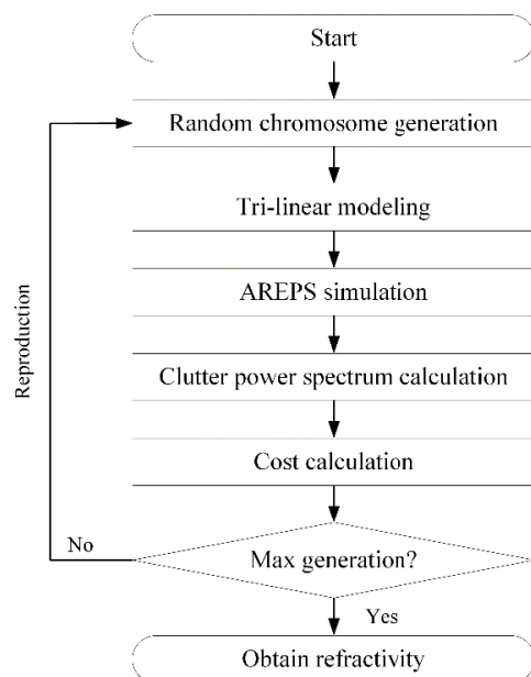
Figure 13. GA process for estimating atmospheric refractivity [378].
