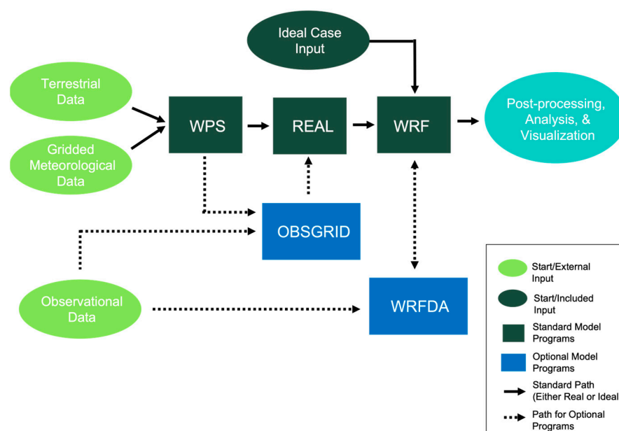
Figure 10. Flow chart of WRF modeling system, where WPS, REAL, OBSGRID and WRFDA denote WRF Preprocessing System, Real Initialization Programs, Observation Grid Module and WRF Data Assimilation, respectively. The step “Post-processing, Analysis, & Visualization” in the diagram marks the end of WRF runs, enabling extraction of WRF outputs, variable derivation and visualization, which transform raw data into intuitive charts and useful analytical results.
