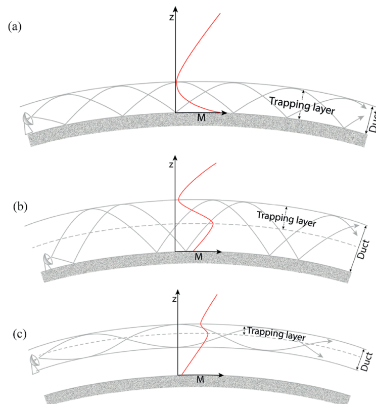
Figure 3. Illustration of the propagation of EM waves from a radar source in various refractive conditions over a distance beyond the line of sight over the Earth. The corresponding vertical M profiles are overlaid on the propagation path: (a) evaporation duct, (b) surface-based duct, and (c) elevated duct [65].
