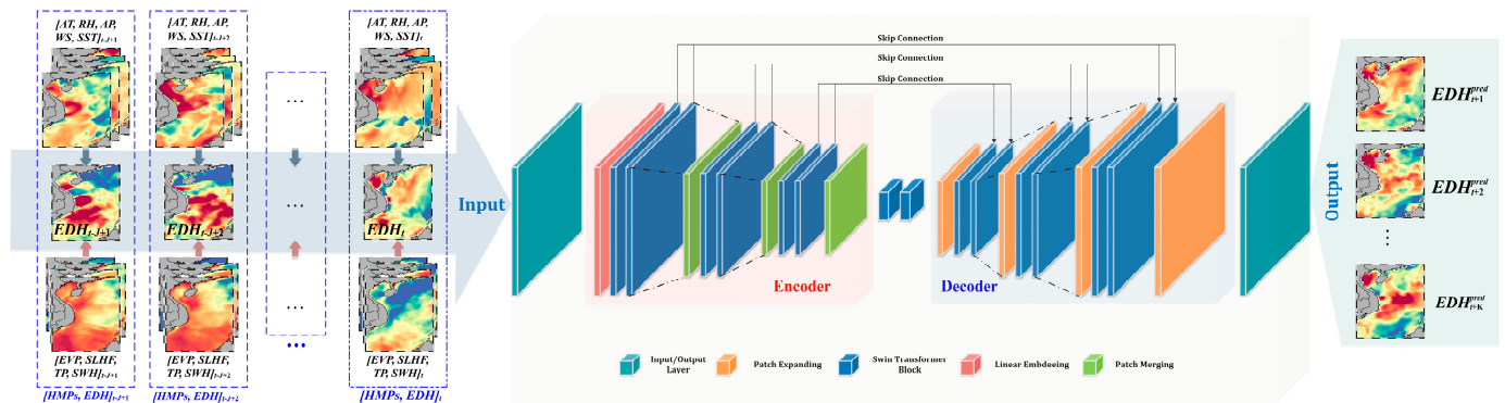
Figure 11. EDH-STNet [189]. This model takes the spatial distribution of EDH at historical times as input and is used to predict the EDH distribution at future times. To improve prediction accuracy, the model also incorporates AT, RH, AP, WS, SST, evaporation (EVP), surface latent heat flux (SLHF), total precipitation (TP), and sufficient wave height (SWH) as supplementary inputs. After the above input is fed into the Swin-Unet model, it is first processed by the encoder: the Swin-Transformer module in the encoder can extract and abstract features from the input data. The above processing module can effectively capture spatial information while deepening the understanding of temporal features. Next, the decoder uses upsampling techniques to gradually reconstruct the advanced features extracted by the encoder, restore detailed information, and ultimately generate an output that is consistent with the original input data. In addition, in the EDH-STNet model, skip connections are used to integrate the features of different levels of the encoder with the features upsampled by the decoder.
