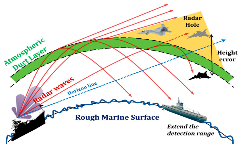
Figure 1. Schematic of atmospheric duct effects on EM waves. This phenomenon extends the operational range of communication systems and enables radar-based BLOS detection of low-altitude targets. Concurrently, the trapping of EM waves within the duct creates an EM shadow zone above the duct layer, where minimal radio energy penetrates due to restricted ray propagation.
