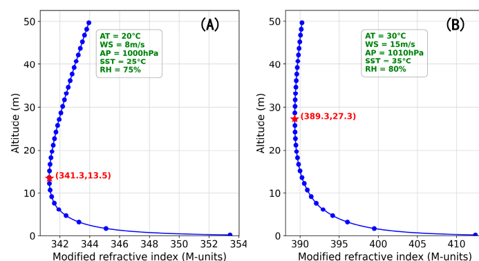
Figure 7. Evaporation duct M -profiles for EDH cases: (A) 13.5 m and (B) 27.3 m [363].
