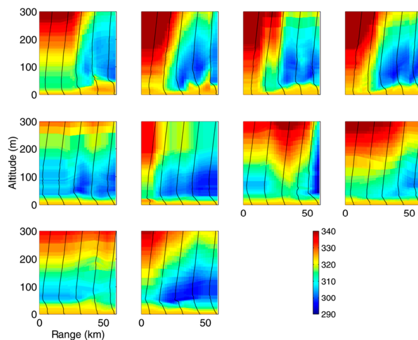
Figure 15. Chronologically ordered M profiles from Wallops ‘98 experiment. The first row is observed from 8:47 to 10:26 EST (08:47–09:05, 09:07–09:32, 09:33–09:57, and 09:58–10:26), the middle from 12:26 to 14:15 EST (12:26–12:50, 12:52–13:17, 13:19–13:49, and 13:51–14:14), and the bottom from 16:00 to 16:52 EST (15:59–16:27 and 16:29–16:52) [31].
