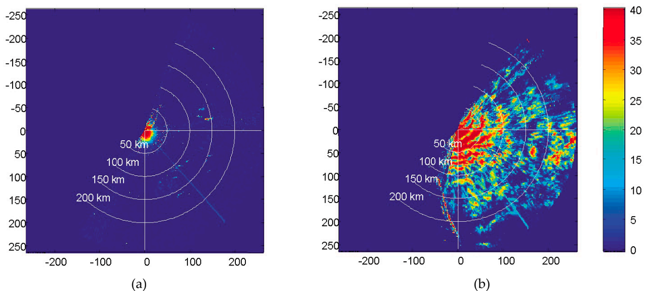
Figure 12. Radar PPI screen showing clutter map (dB) during the 1998 SPANDAR experiment resulting from a (a) weak evaporation duct, (b) surface-based duct [32].
