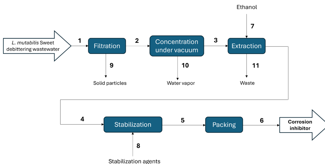
Figure 3. Production plant for a corrosion inhibitor based on L. mutabilis debittering wastewater: block diagram (BD).
