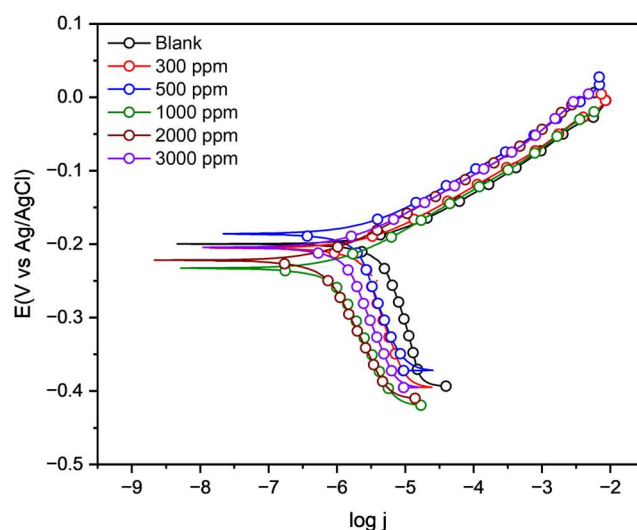
Figure 2. Potentiodynamic polarization performance of L. mutabilis extract E6 in 0.5 M HCl in the absence and addition of varying concentrations of E6 green inhibitor at 298 K.
