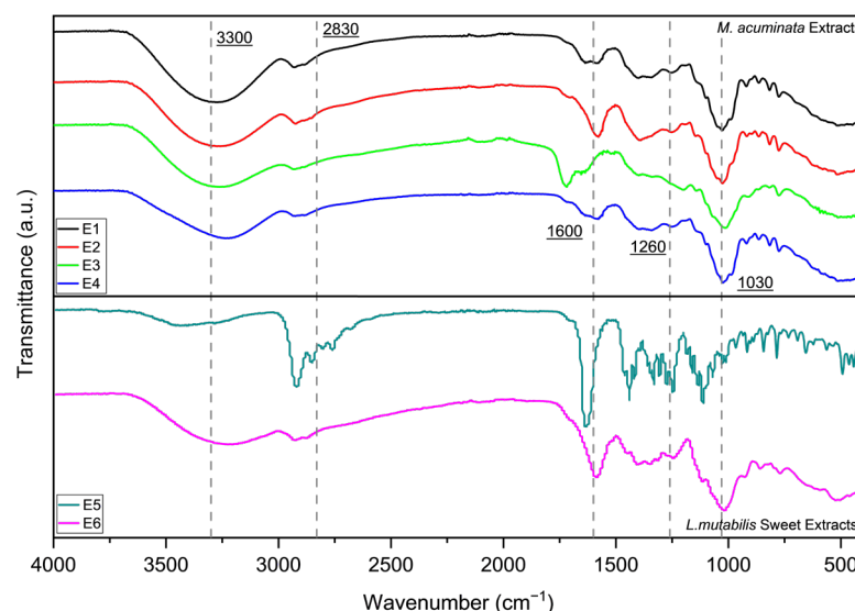
Figure 1. FTIR spectrum of M. acuminata peel and L. mutabilis extracts.
