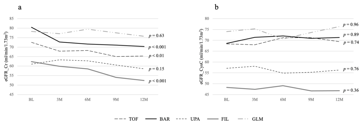
Figure 1. Estimated glomerular filtration rate (eGFR) from baseline over one year at every three months. Symbols on the right of each graph show the statistical significance ( p -value) in the trend of eGFR in each drug group. There was no significant difference in eGFR across all pairs of groups at any time point. (a): eGFR based on creatinine. (b): eGFR based on cystatin C.
