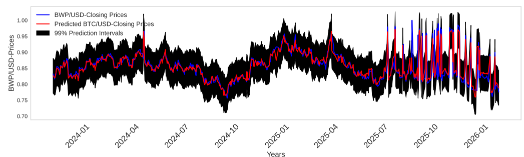
Figure 4. Prediction interval widths without transfer learning.
