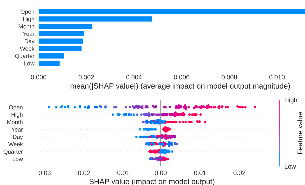
Figure 8. SHAP values for feature importance.
