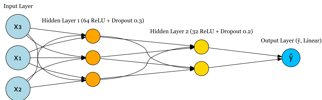
Figure 2. Proposed DNN architecture. Source: authors' own computation.
