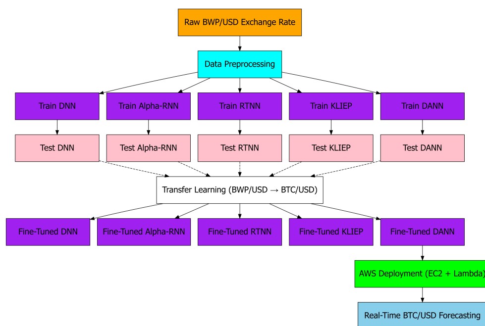
Figure 1. Workflow of the proposed transfer learning framework. The DNN, Alpha-RNN, RTNN, KLIEP, and DANN are trained and tested on BWP/USD data before applying transfer learning to BTC/USD. The fine-tuned models are deployed on AWS for real-time exchange rate forecasting. Source: Authors' own computation.
