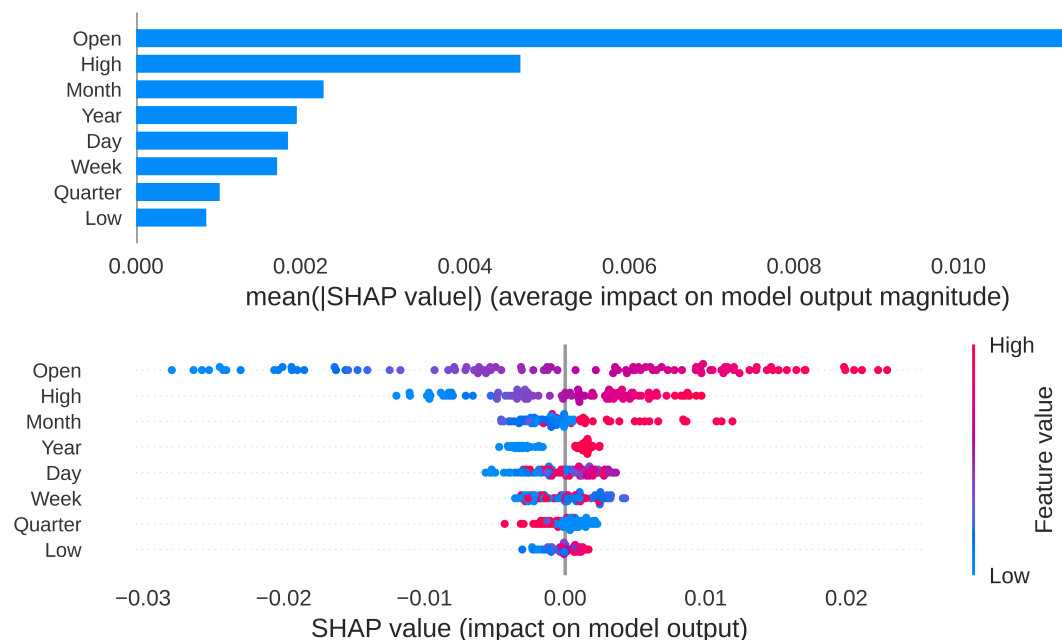
Figure 5. SHAP values for feature importance for BWP/USD.
