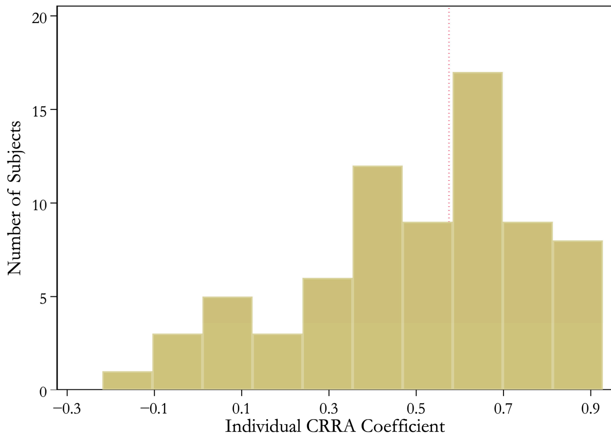
Figure 3. Individual CRRA coefficients r_i from observed choices under EUT specification VI.
