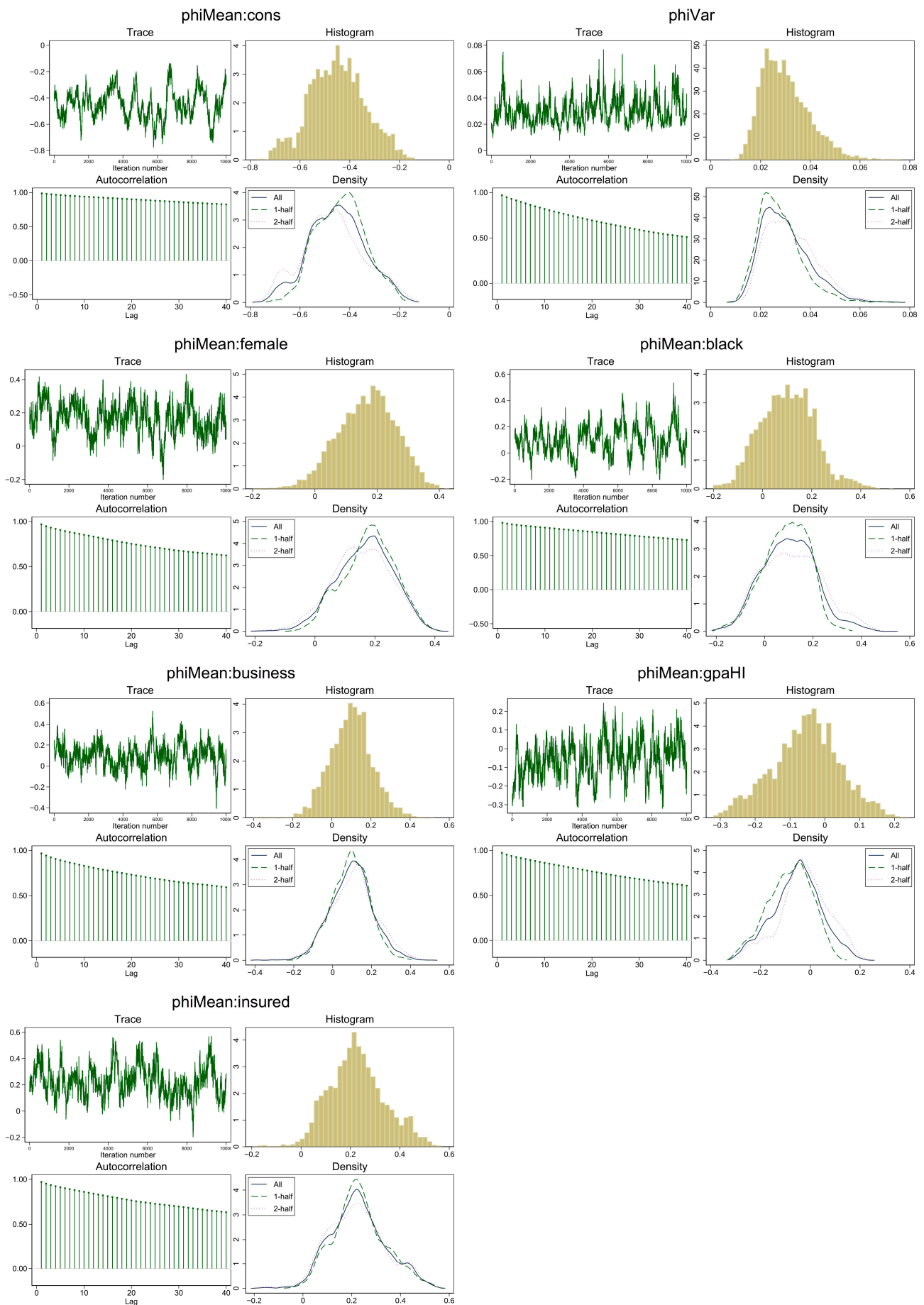
Figure A1. Diagnostic plots of demographic coefficients of \phi in RDU specification VI.
