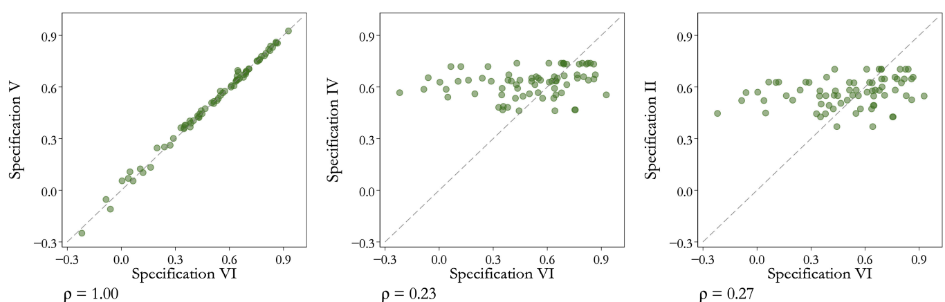
Figure 4. Individual CRRA coefficients r_i from observed choices under different EUT specifications.
