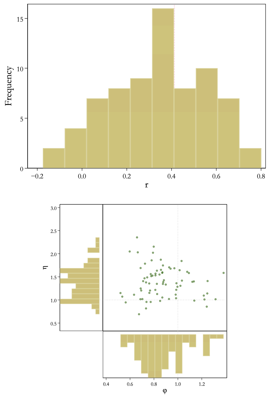
Figure 5. Posterior means of individual estimates assuming Specification V of the RDU Prelec model.
