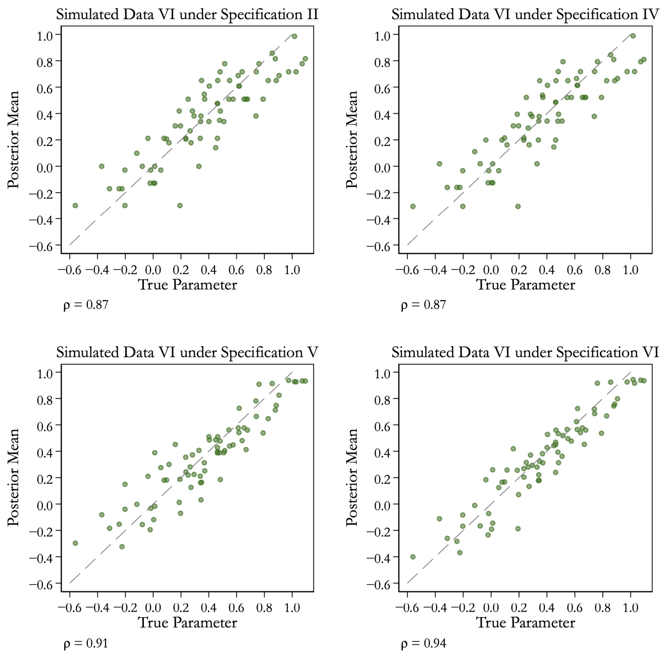
Figure 2. Individual CRRA coefficients using simulated dataset VI assuming incorrect specifications.
