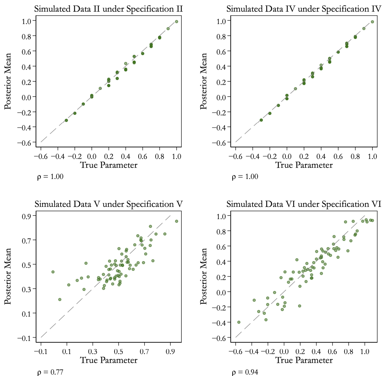
Figure 1. Individual CRRA coefficients in simulated data estimation.
