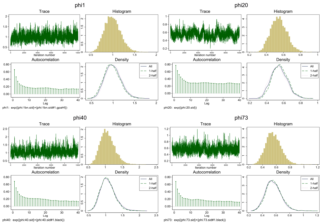
Figure A2. Diagnostic plots of individual \phi of subjects 1, 20, 40 and 73 in RDU specification VI.
