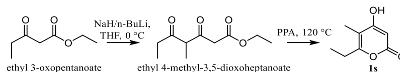
Scheme 1. Synthesis of 6-Ethyl-4-hydroxy-5-methyl- \alpha -pyrone 1s .
