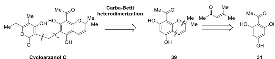
Scheme 13. Proposed retrosynthetic analysis of cycloarzanol C [2,26].
