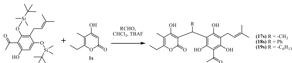
Scheme 7. Synthesis of 1'-methylarzanol 17s , 1'-phenylarzanol 18s , and 1'-hexylarzanol 19c .
