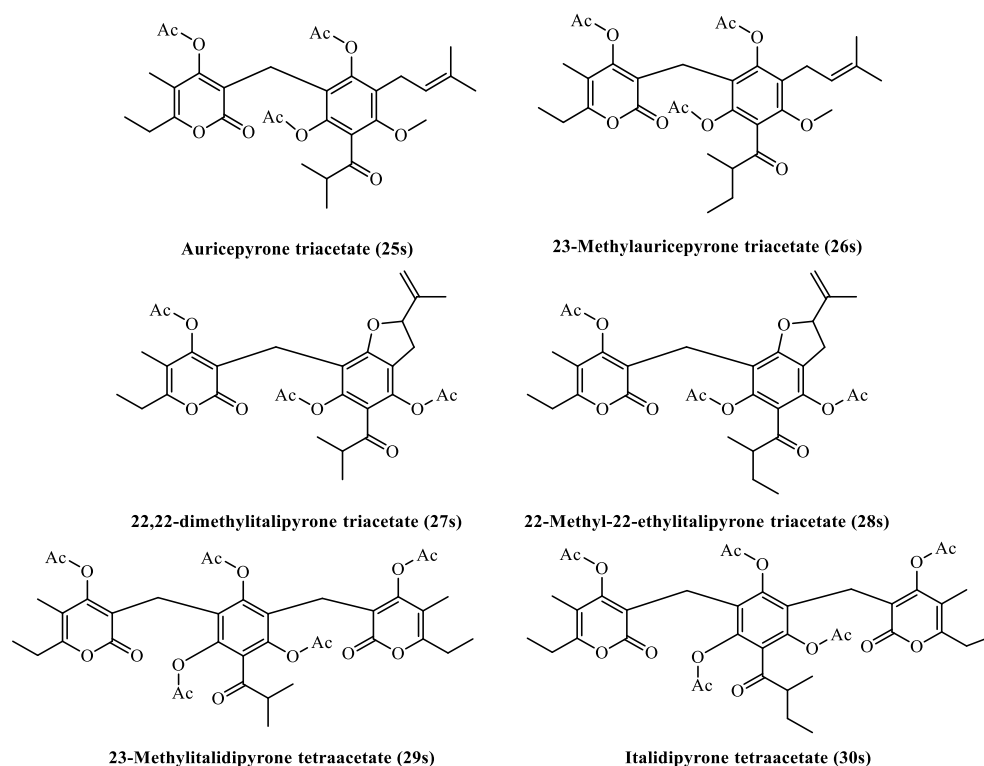
Figure 2. Structural formulas of compounds acetyl derivatives of phloroglucinol- \alpha -pyrones.
