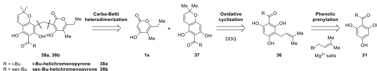
Scheme 12. Proposed retrosynthetic analysis of helichromenopyrone-type chromene heterodimers [2,22,25].
