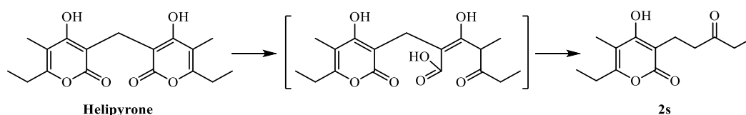
Scheme 2. Synthesis of 6-ethyl-4-hydroxy-5-methyl-3-(3-oxopentyl)-2H-pyran-2-one 2s .
