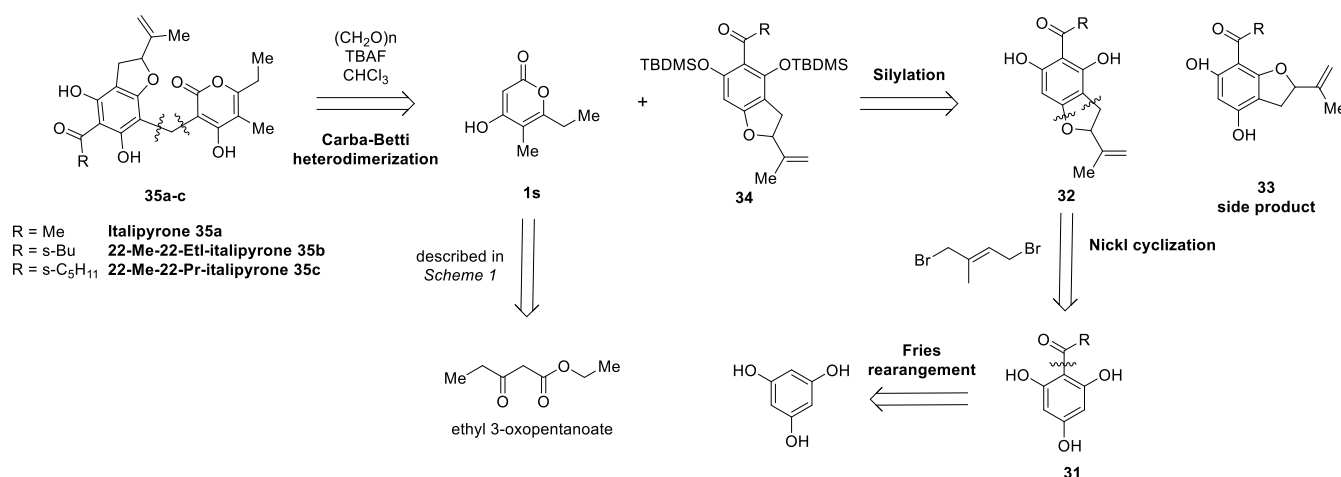
Scheme 10. Proposed retrosynthetic analysis of italipyron-type benzofurane-2-pyrone heterodimers [2,21,22].
