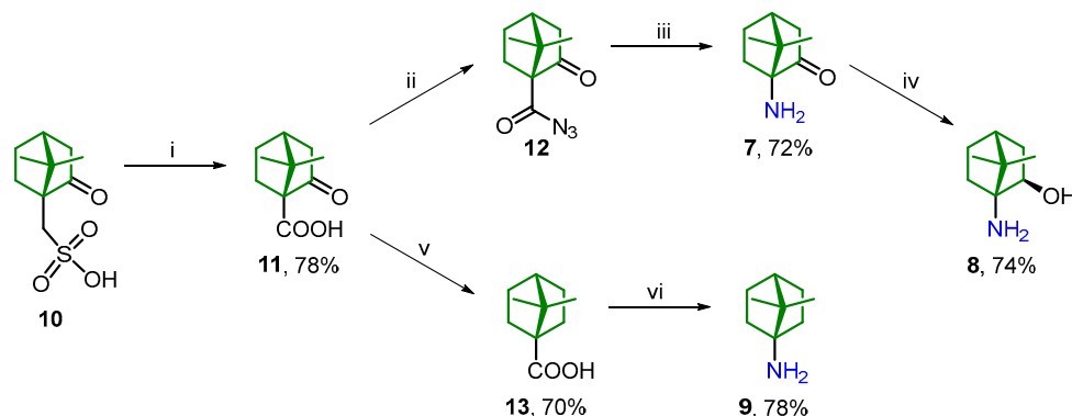
Scheme 3. Synthesis of amines 7–9. Reagents and conditions: (i) (1) \text{SOCl}_2 , reflux, 3 h, (2) \text{KMnO}_4 , \text{Na}_2\text{CO}_3 , 80 °C, 2 h; (ii) (1) \text{SOCl}_2 , reflux, 3 h, (2) \text{NaN}_3 , acetone/ \text{H}_2\text{O} , 1 h; (iii) (1) toluene, reflux, 3 h, (2) \text{H}^+ , reflux, 8 h; (iv) \text{NaBH}_4 , \text{CeCl}_3 \cdot 7\text{H}_2\text{O} , \text{MeOH} , -30 °C, 4 h; (v) \text{N}_2\text{H}_4 \cdot \text{H}_2\text{O} , \text{KOH} , reflux, 8 h; (vi) \text{H}_2\text{SO}_4 , \text{NaN}_3 , 50 °C, 1 h.
