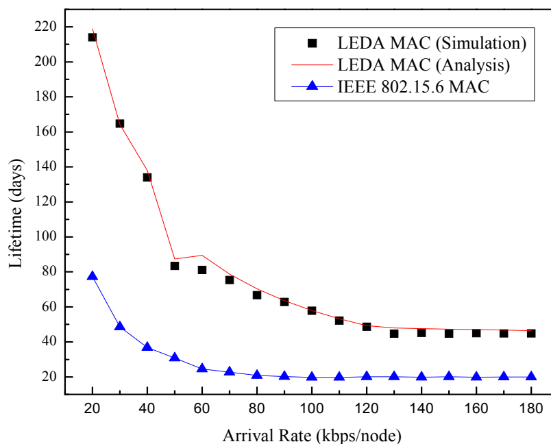
Figure 18. Lifetime of network vs. arrival rate.
