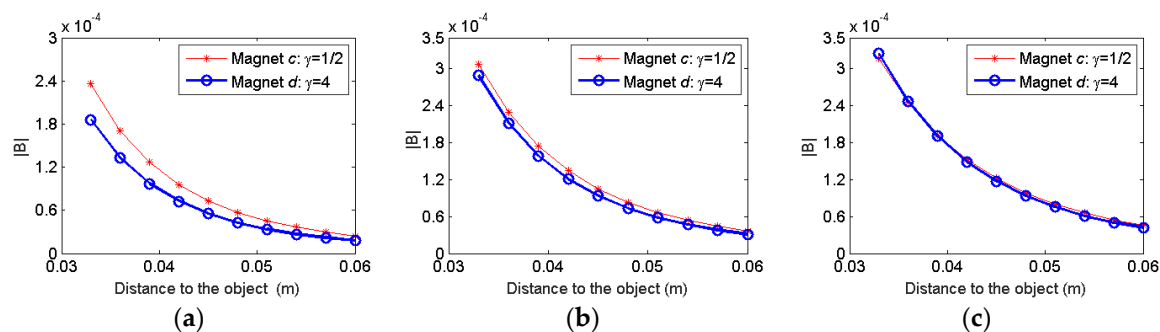
Figure 10. Comparison of the distortion field when magnets with doubled volume and different aspect ratios are used: (a) W = 2 cm; (b) W = 4 cm; (c) W = 6 cm.
