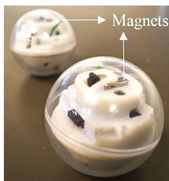
Figure 13. VIRGO robot integrated with the embedded magnetic proximity sensor.
