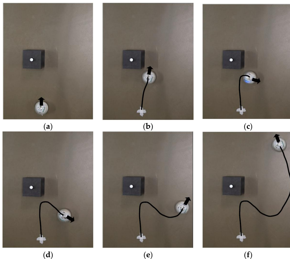
Figure 21. Snapshots of the robot course as it detects and avoid the obstacle while still reaching its target waypoint: (a) Robot starts moving; (b) Robot moves closer to the obstacle and detects its presence; (c) Robot turns clockwise after detecting the obstacle; (d) Robot adjusts its course towards the intermediate waypoint; (e) Robot adjusts the course again to reach its original target waypoint; (f) Robot approaches the target waypoint.
