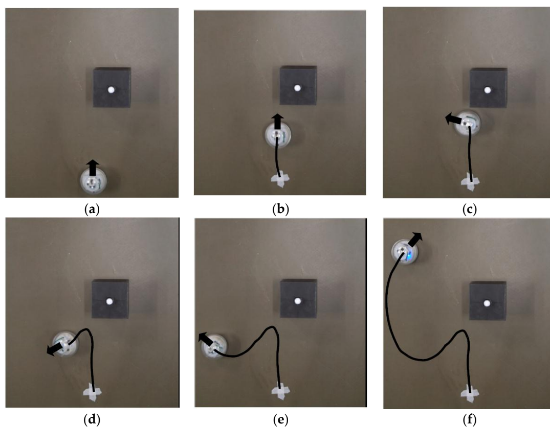
Figure 19. Snapshots of the robot course as it detects and avoids the obstacle while still reaching its target waypoint: (a) Robot starts moving; (b) Robot moves closer to the obstacle and detects its presence; (c) Robot turns counterclockwise after detecting the obstacle; (d) Robot adjusts its course towards the intermediate waypoint; (e) Robot adjusts the course again to reach its original target waypoint; (f) Robot approaches the target waypoint.
