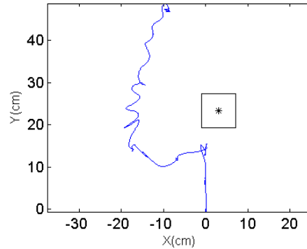
Figure 20. Trajectory from the VICON system.
