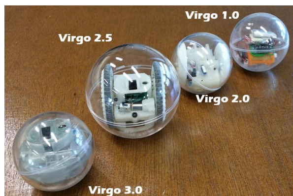
Figure 1. VIRGO, a spherical robot developed in SUTD [17].
