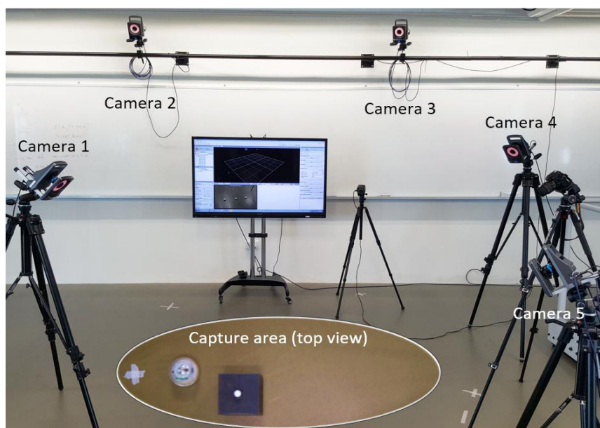
Figure 14. Experimental setup in the VICON system.
