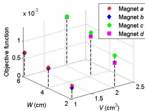
Figure 12. Comparison of the objective functions for different magnets.
