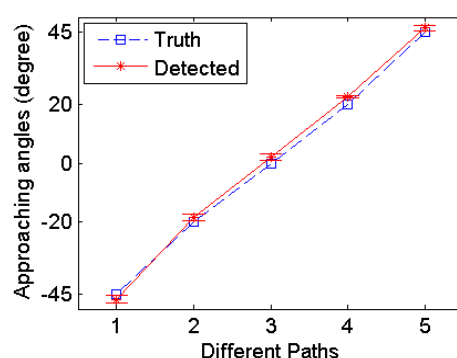
Figure 15. Angle detection accuracy along different approaching paths.
