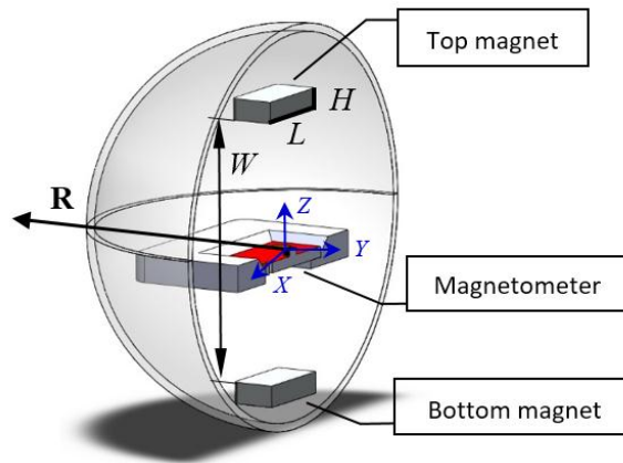
Figure 6. Geometric parameters of the magnetic proximity sensor.
