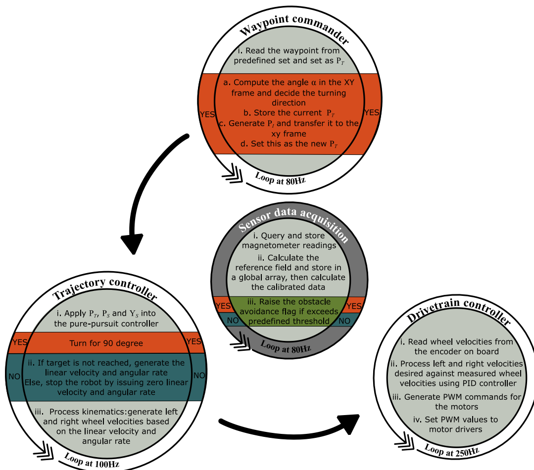
Figure 8. Illustration of the detailed algorithm.
