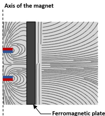
Figure 3. Distorted field pattern due to an approaching object.
