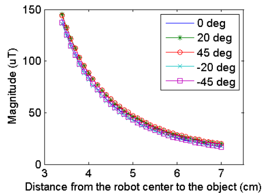
Figure 16. Relation between the measured field and the distance to the ferromagnetic object.
