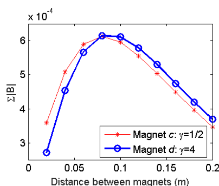
Figure 11. Effect of the distance between two magnets on the distortion field strength.
