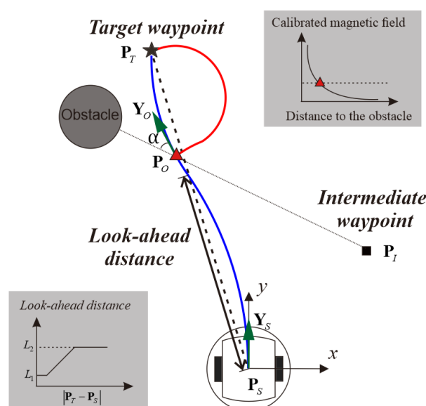
Figure 7. Illustration of the pure-pursuit method and obstacle avoidance behavior integration.
