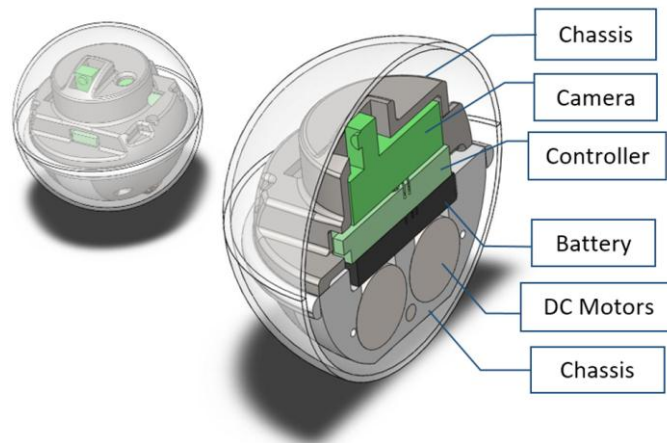
Figure 5. Configuration of VIRGO.
