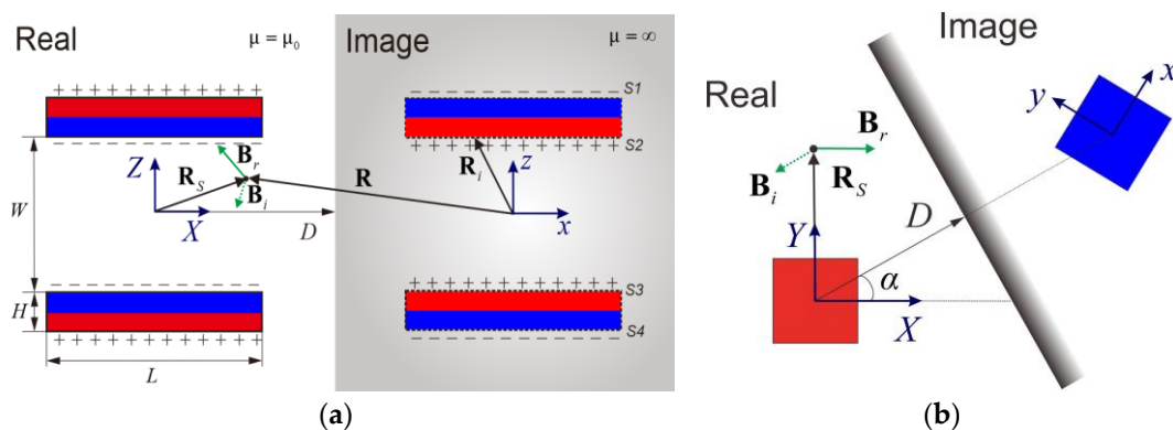
Figure 4. Modeling of the approaching obstacle as image charges: (a) approaching angle \alpha = 0 ; (b) approaching angle \alpha \neq 0 .
