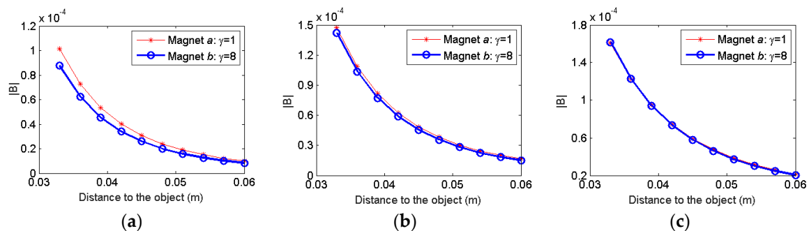
Figure 9. Comparison of the distortion field when magnets with different aspect ratios are used: (a) W = 2 cm; (b) W = 4 cm; (c) W = 6 cm.
