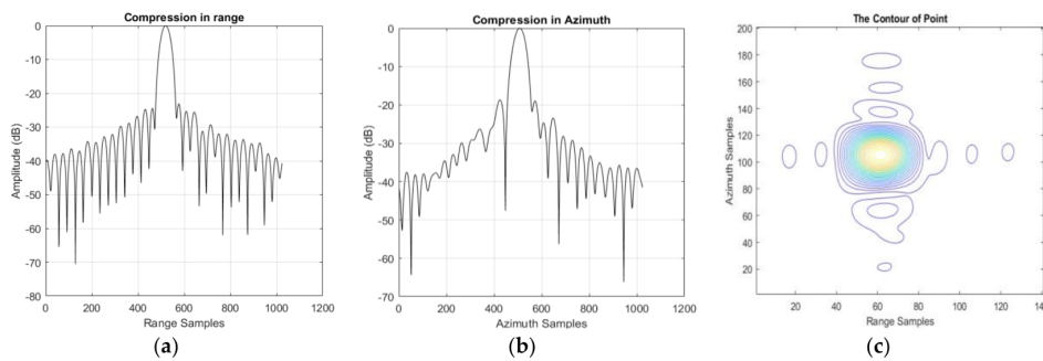
Figure 9. The compression result after stop-and-go correction. (a) The compression result of the corner reflector in slant range; (b) The compression result of the corner reflector in azimuth; (c) The two-dimension contour in azimuth and slant range.
