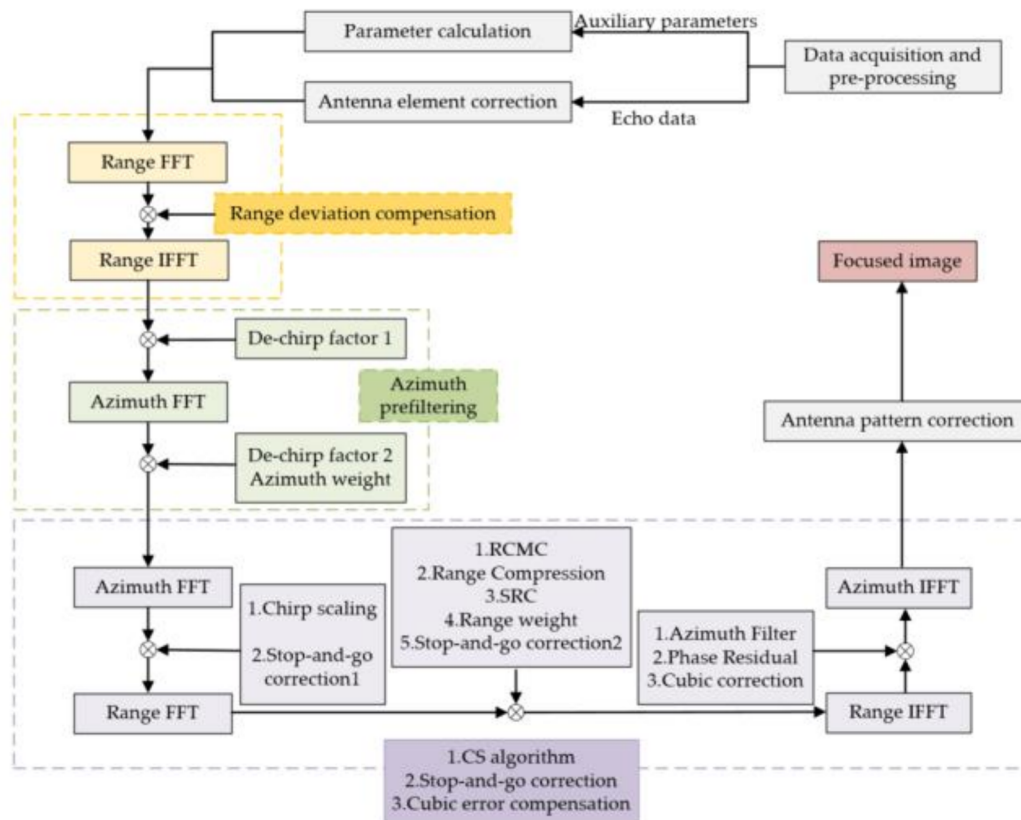
Figure 5. Data processing flow of GF-3 in ST mode.
