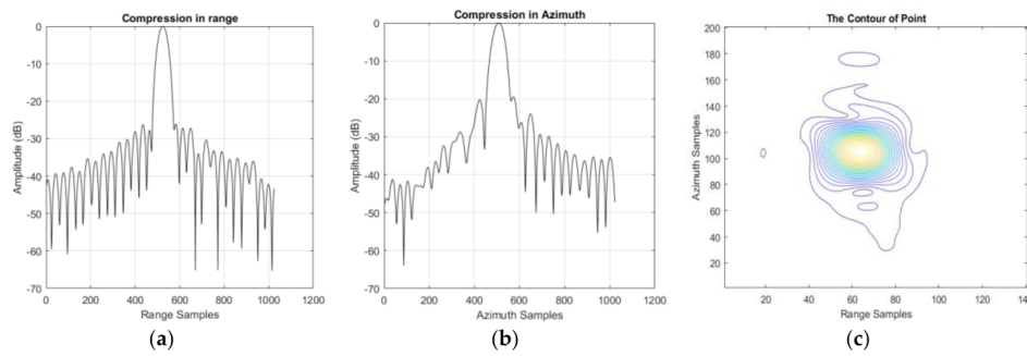
Figure 8. The compression result after model error correction. (a) The compression result of the corner reflector in slant range; (b) The compression result of the corner reflector in azimuth; (c) The two-dimension contour in azimuth and slant range.
