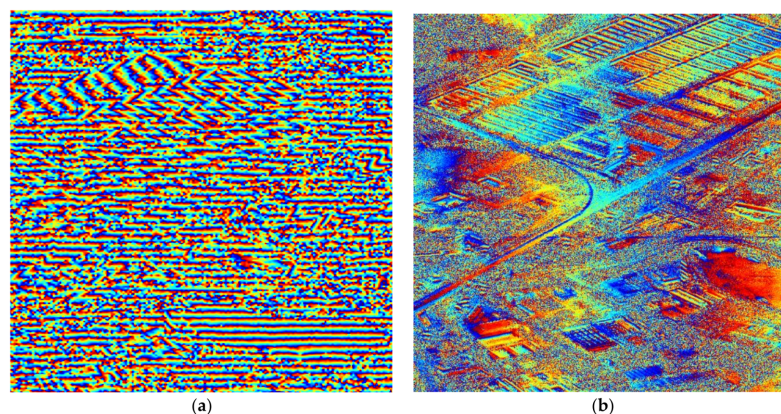
Figure 11. Some results of repeat-pass SAR interferometry experiment. (a) The interferogram of the spot marked with the white box in Figure 10; (b) The flattened interferogram of (a).
