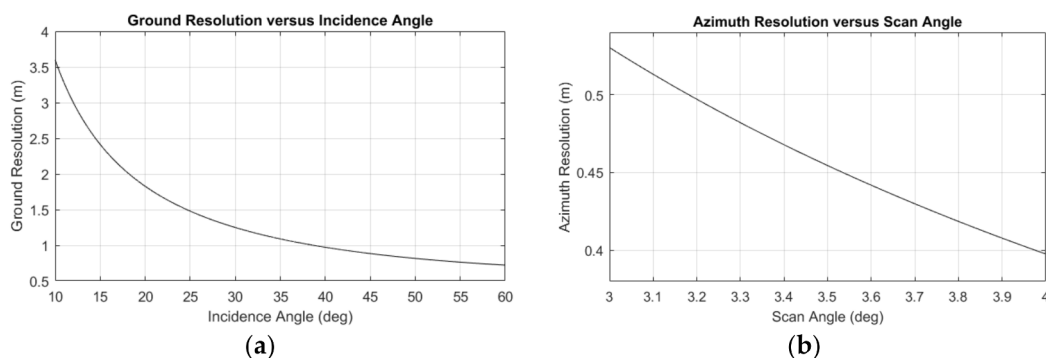
Figure 1. The resolution in ST mode. (a) The ground resolution versus the incidence angle; (b) The azimuth resolution versus the scan angle range.
