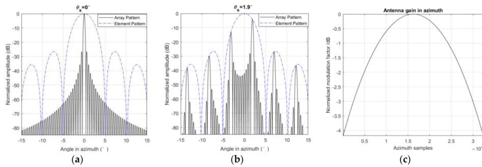
Figure 3. Antenna pattern of GF-3. (a) The antenna pattern when \theta_s = 0^\circ ; (b) The antenna pattern when \theta_s = 1.9^\circ ; (c) The normalized modulation factor of GF-3 antenna gain in azimuth in this experiment.
