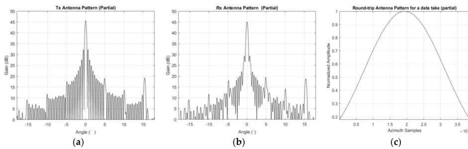
Figure 4. GF-3 azimuth antenna pattern of the data acquired in this experiment. (a) The antenna pattern within [-18^\circ, 18^\circ] in transmit mode; (b) The antenna pattern within [-18^\circ, 18^\circ] in receive mode; (c) The interpolated round-trip antenna pattern.
