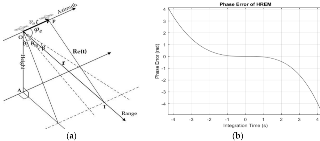
Figure 2. Schemes of hyperbolic range equivalent model (HREM): (a) The geometric figure of the HREM; (b) The model error between the actual range history and the equivalent range history in the ST experiment.
