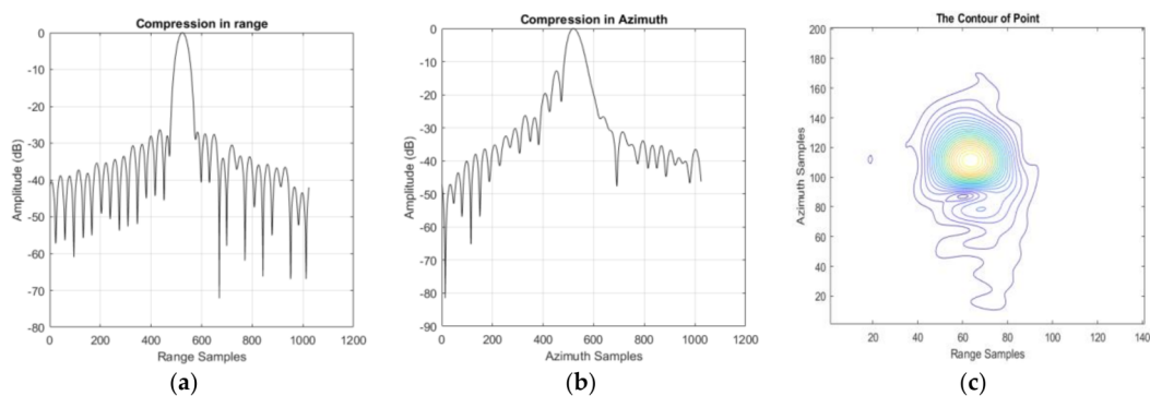
Figure 7. The compression result of the corner reflector processed by the two-step processing algorithm. (a) The compression result of the corner reflector in slant range; (b) The compression result of the corner reflector in azimuth; (c) The two-dimension contour in azimuth and slant range.
