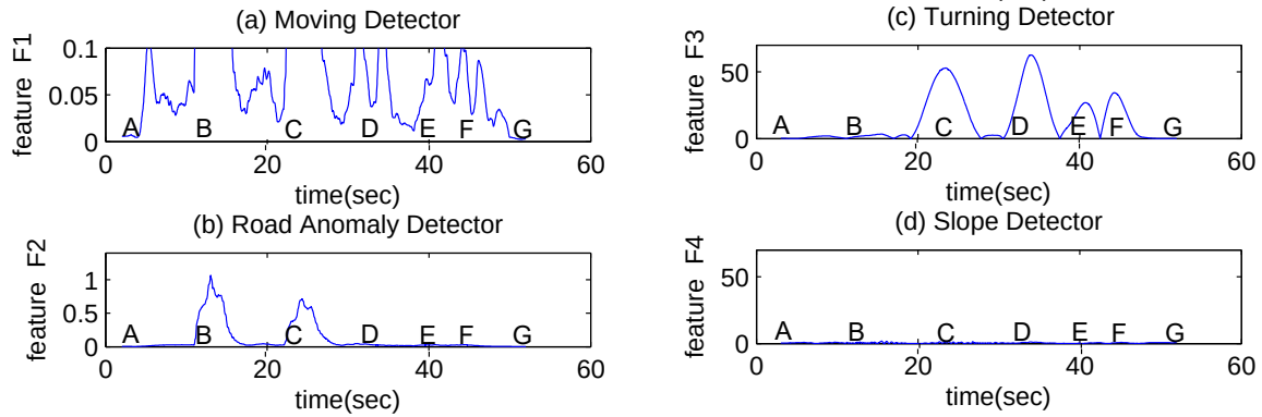
Figure 4. Features calculated for different detectors.
