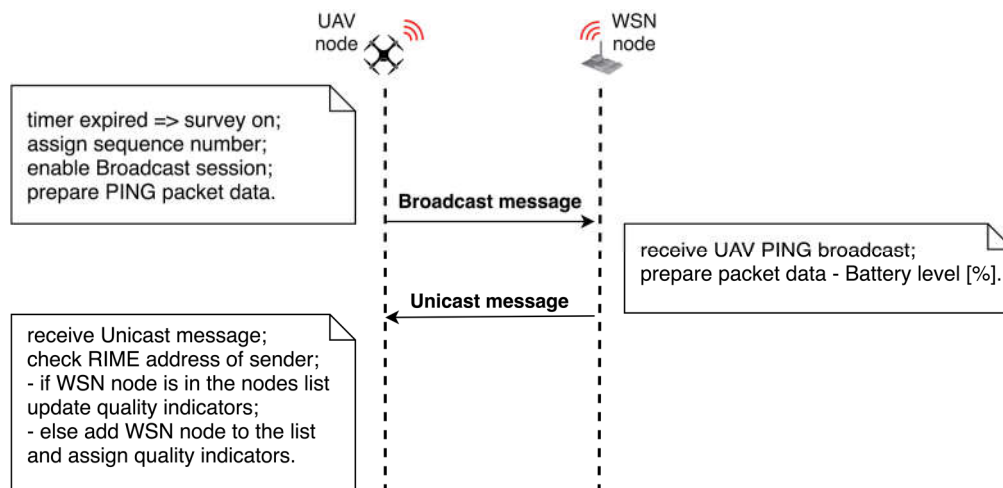
Figure 6. UAV-WSN survey dialog sequence.
