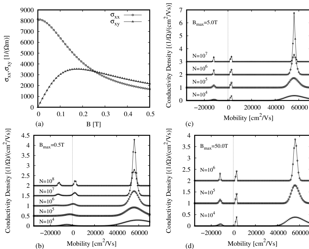
Figure A1. Mobility spectrum calculated for different parameters N , \delta B and B_{max} , as described in the text.
