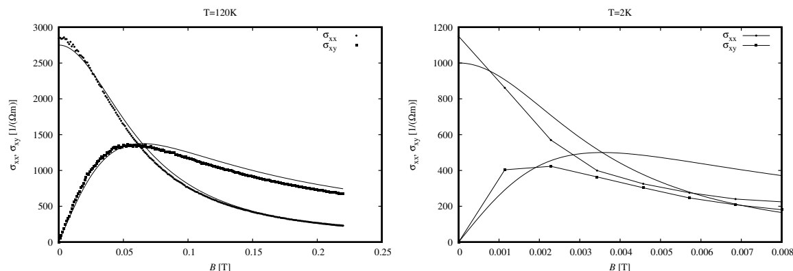
Figure 4. Components of the conductivity tensor at 120 K ( left ) and 2 K ( right ). Points: experimental results; smooth solid lines—fits of Equation (1) with N = 1 . Note a different range of B in the two panels.
