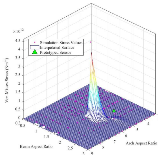
Figure 8. Von-Mises stress vs. structural design parameter study for the cylindrical arch spring.
