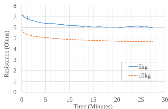
Figure 24. Experiment results: sensor drift plot—resistance change over the time.
