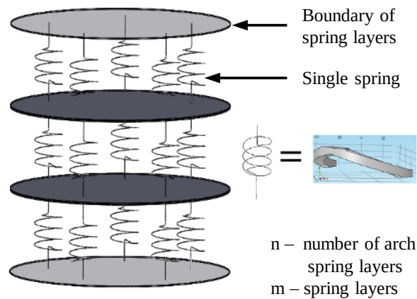
Figure 4. Cylindrical arch spring structure was analytically modelled for further modifications.
