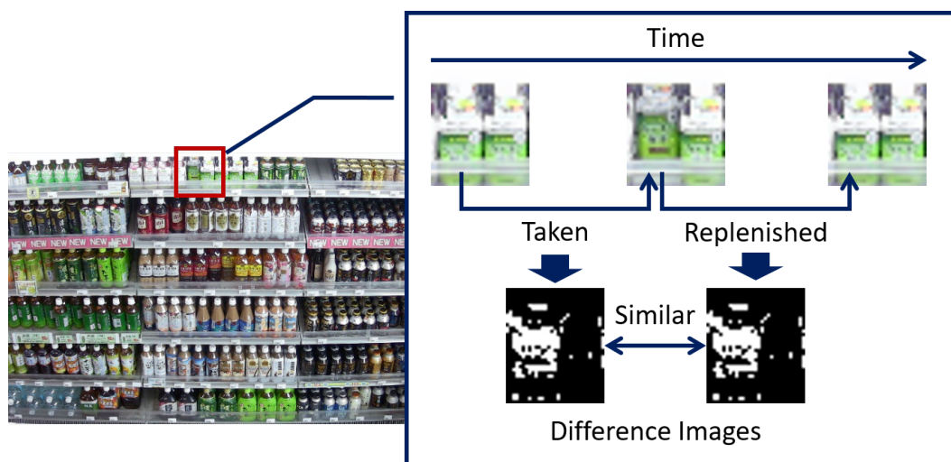
Figure 6. Examples of difference images for change regions of “product taken” and “product replenished”.
