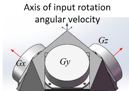
Figure 1. Structure of IMU based on RLG in rate-biased mode.
