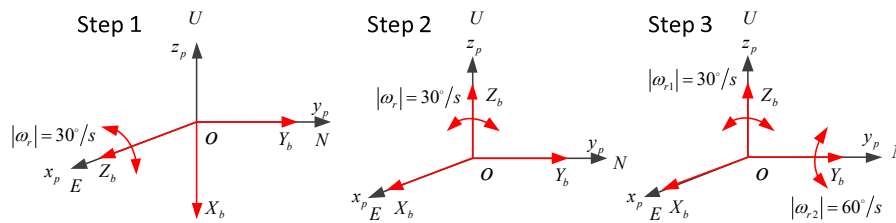
Figure 5. Three steps of the calibration.
