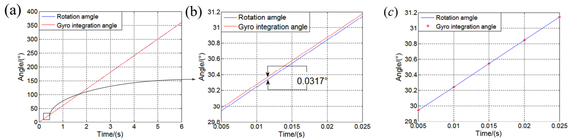
Figure 9. Unsynchronized time compensation results. (a) Before compensation; (b) Partial enlargement of (a); (c) Results after compensation.
