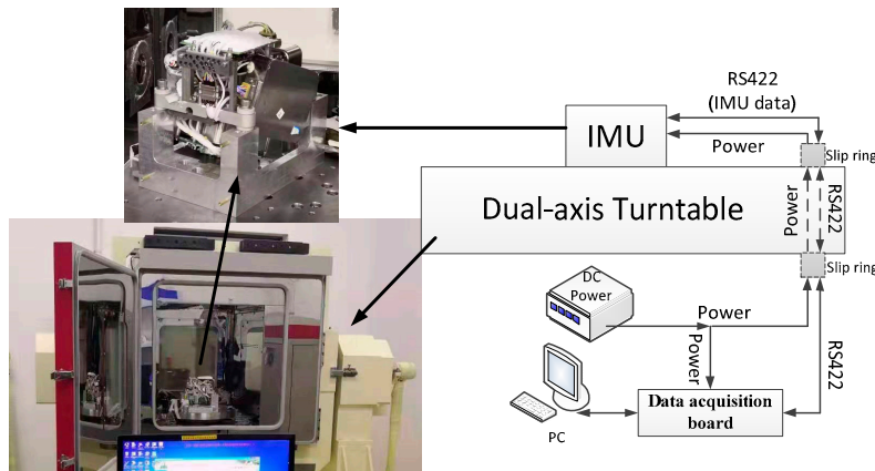
Figure 3. Experimental setup.
