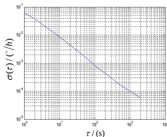
Figure 13. Root Allan variance versus averaging time for gyro in rate-biased mode.
