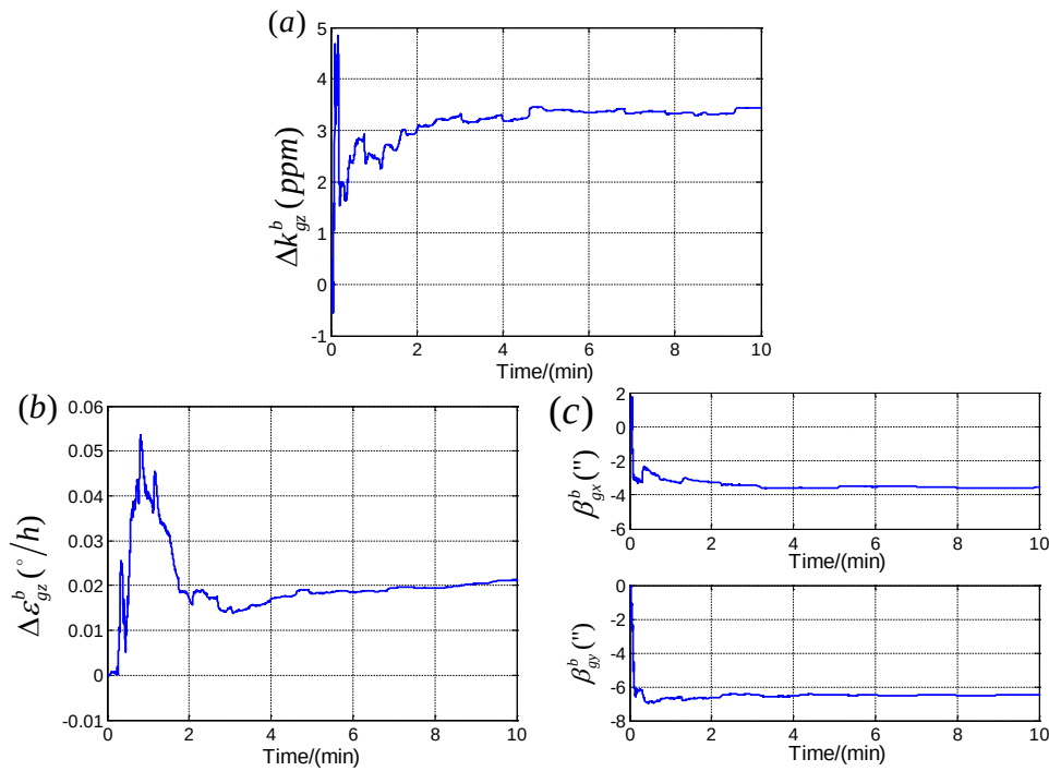
Figure 6. The curve convergences of the calibrated errors in the first step. (a) The curve convergences of \Delta k_{g_z}^b ; (b) The curve convergences of \varepsilon_{g_z}^b ; (c) The curve convergences of \beta_{g_x}^b and \beta_{g_y}^b .
