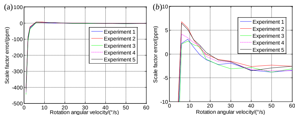
Figure 4. \Delta k_{gz}^b of the IMU in rate-biased mode; (a) \Delta k_{gz}^b with the change of the rotation angular velocity; (b) Partial enlargement of (a).
