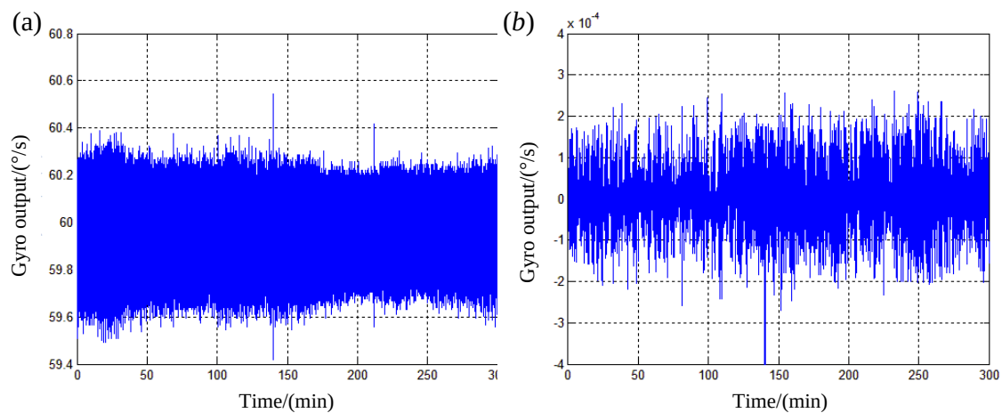
Figure 12. Gyro outputs for calculating ARW. (a) Original gyro outputs; (b) Gyro outputs after pre-processing.
