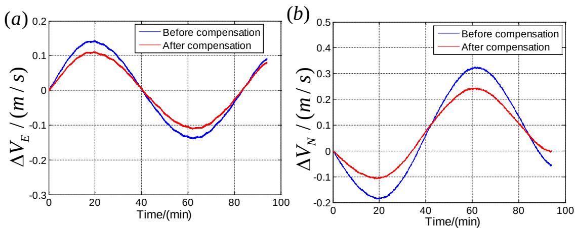
Figure 7. Navigation results before and after compensating the calibration results. (a) Velocity errors in east direction compensation; (b) Velocity errors in north direction.
