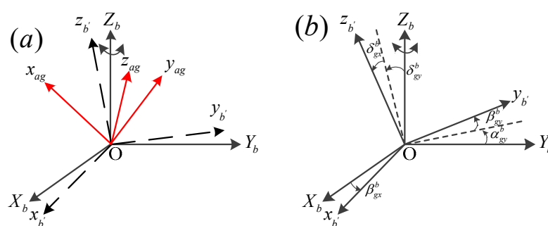
Figure 2. Frames of the IMU. (a) The relationship between a frame, b frame and b' frame; (b) The errors angles between b frame and b' frame.
