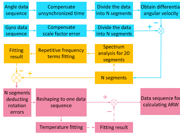
Figure 8. Flow of the process.
