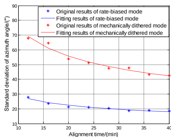
Figure 14. Fitting results of standard deviation of azimuth angle verse T in alignment experiments.
