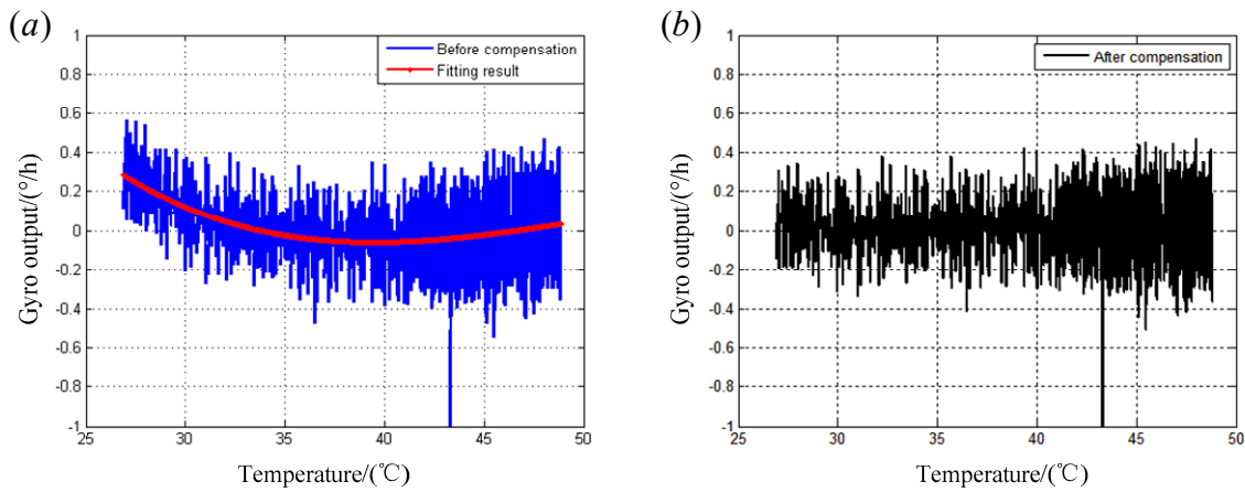
Figure 11. Temperature compensation result; (a) The fitting result of the data; (b) The result after temperature compensation.
