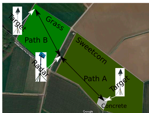
Figure 6. Illustration (from Google Earth) of the experimental setup in the fields of Wachtberg. Two different propagation paths were measured with the same radar and the same standard target. Sweetcorn was grown in the field of propagation path A (186 m), whereas grass was grown on the field of propagation in path B (159 m).
