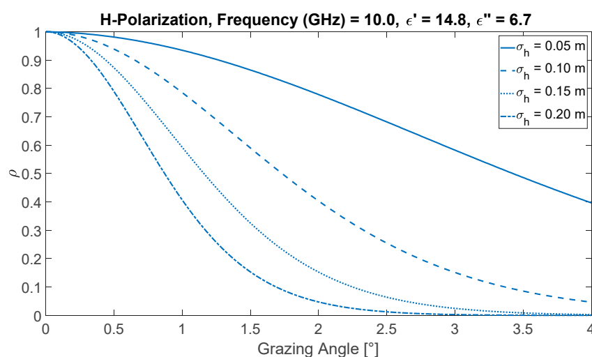
Figure 2. Modulus of the reflection coefficient \rho (X band, horizontal polarization) for soil (clay) with moisture of 35 g/cm 3 , low grazing angles, and four values of \sigma_h .
