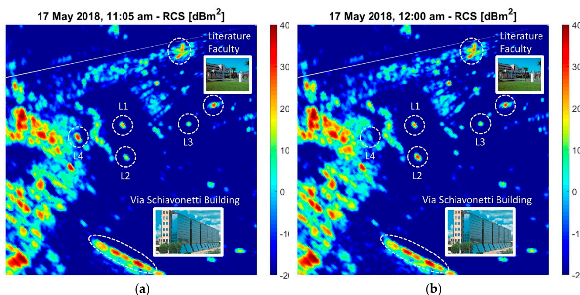
Figure 10. Measured RCS, 17 May 2018: (a) 11:05 and (b) 12:00.
