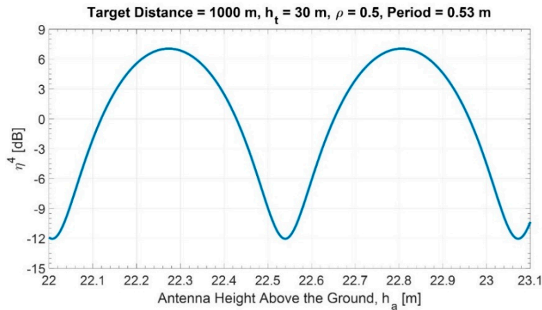
Figure 3. Multipath factor \eta^4 vs. the antenna height (target distance D = 1000 \text{ m} and target height of h_t = 30 \text{ m} ). The period \frac{\lambda D}{2h_t} is equal to 0.53 \text{ m} .
