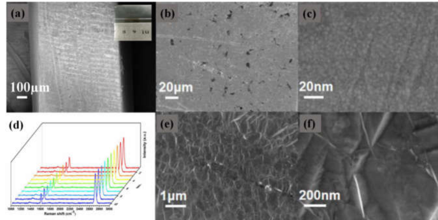
Figure 3. (a) The SEM of new D-shape area morphology. (b) The SEM image of the D-type area. (c) The SEM image of the gold film. (d) 10 groups of fixed-point scanning Raman spectra on the same sample. (e) The SEM image of grown graphene. (f) The SEM image of graphene folds after magnification.
