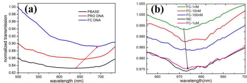
Figure 8. (a) The normalized transmission spectra after the addition of PBASE, probe DNA and tDNA to the D-type region. (b) The normalized transmission spectra of different concentrations of full complementary (FC) and non-complementary (NC) DNA.
