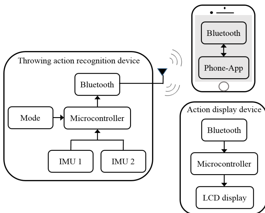
Figure 1. System architecture.
