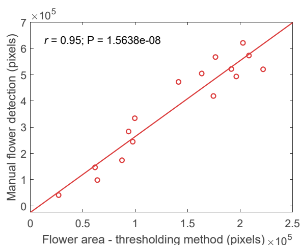
Figure 5. Correlation between flowers detected by thresholding method and manual identification.
