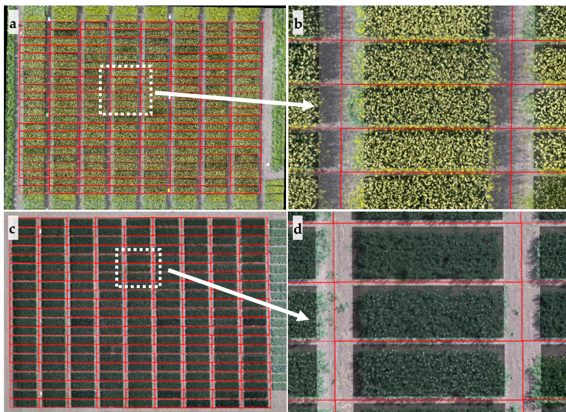
Figure 4. Results of flower extraction from aerial images of spring canola and pea. Separated individual plots for spring canola and pea are outlined by red rectangles as shown in (a) and (c), respectively; regions of interest (plot with four edges removed) were dimmed while flowers were highlighted in white as shown in (b) and (d); (b) and (d) are zoom-in images of white-highlighted areas of (a) and (c), respectively.
