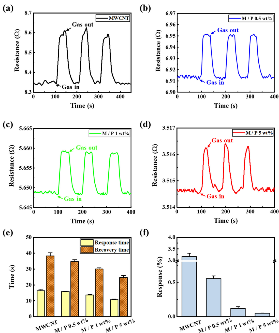
Figure 6. Response curves to 1000 ppm of CO gas for (a) pristine MWCNTs and (b) 0.5 wt% PEDOT:PSS-MWCNTs. (c) 1 wt% PEDOT:PSS-MWCNTs. (d) 5 wt% PEDOT:PSS-MWCNTs. (e)
