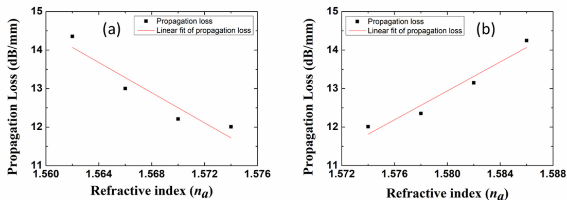
Figure 8. Propagation loss ( MPA_a ) as a function of n_a ; (a) n_a < n_{SU-8} , and (b) n_a > n_{SU-8} .
