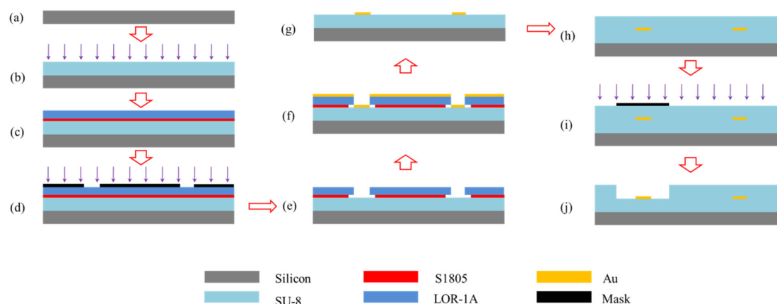
Figure 9. Fabrication process flow of LRSPP waveguide sensors. (a) silicon substrate preparation, (b) spin-coating and curing of SU-8 bottom cladding, (c) LOR-1A and S1805 stack formation, (d) UV photolithography, (e) LOR-1A and S1805 development, (f) Au thermal deposition, (g) double-layer lift-off, (h) spin-coating and curing of SU-8 upper cladding, (i) UV photolithography, (j) development.
