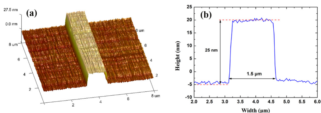
Figure 10. (a) areal scan, and (b) linear scan of an Au stripe on the SU-8 bottom cladding by atomic force microscopy. The Au stripe is 1.5 \mu\text{m} wide and 25 nm high.
