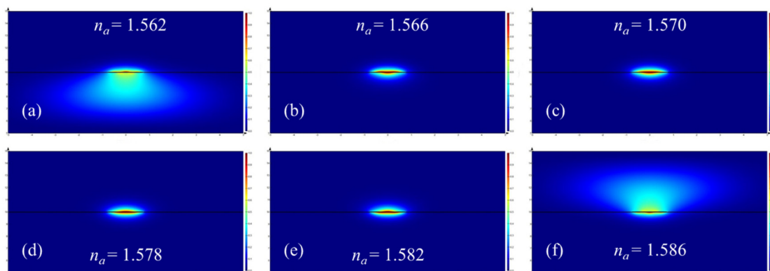
Figure 7. Distribution of the vertical transverse electric field component ( E_y ) of the fundamental LRSP mode for different cases of RI (a) 1.562, (b) 1.566, (c) 1.570, (d) 1.578, (e) 1.582 and (f) 1.586 in the fluidic channel ( n_a ). Here, the width and thickness of the Au stripe are 1.5 \mu\text{m} and 25 nm, respectively.
