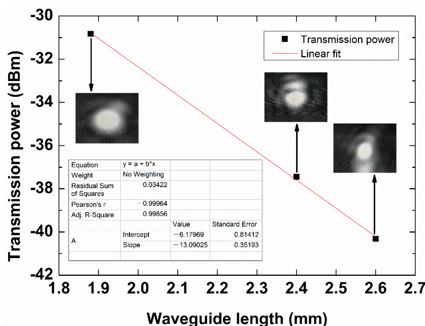
Figure 13. Transmission power as a function of LRSPP waveguide length at optical wavelength 850 nm. Linear fitting of the measured insertion loss of LRSPP waveguides with different lengths yields a mode power attenuation \text{MPA}_w of 13.09 dB/mm at an adjusted R-squared of 0.99856 and a standard deviation of 0.814. Insets show the far field LRSP mode patterns.
