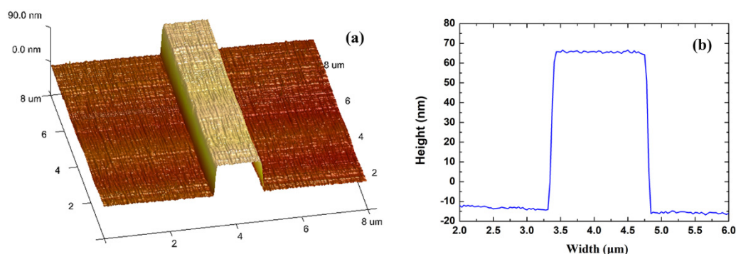
Figure 11. (a) areal scan, and (b) linear scan of an Au stripe by atomic force microscopy after oxygen plasma cleaning, but before application, of the SU-8 upper cladding.
