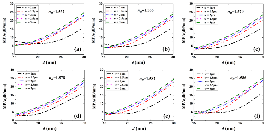
Figure 4. MPA as a function of Au stripe thickness d for different stripe widths w and sensing solutions with n_a of (a) 1.562, (b) 1.566, (c) 1.570, (d) 1.578, (e) 1.582 and (f) 1.586.
