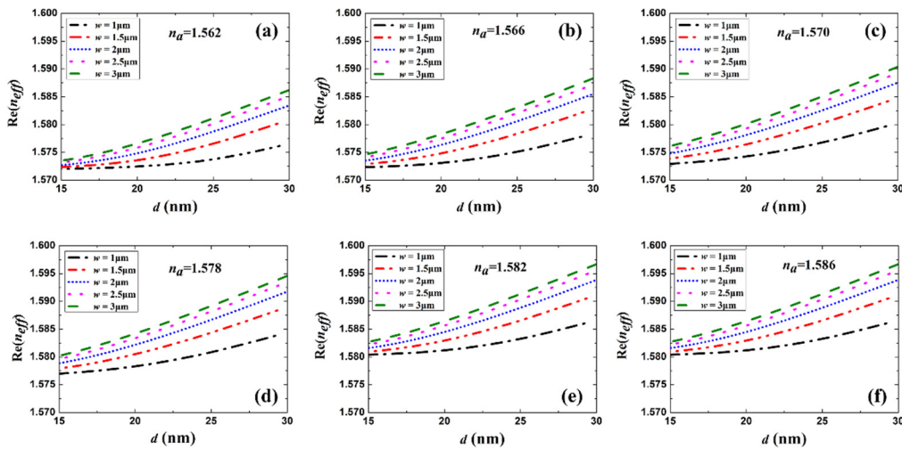
Figure 3. \text{Re}(n_{\text{eff}}) as a function of Au stripe thickness d for different stripe widths w and sensing solutions with n_a of (a) 1.562, (b) 1.566, (c) 1.570, (d) 1.578, (e) 1.582 and (f) 1.586.
