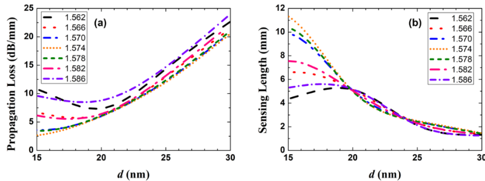
Figure 6. (a) Propagation loss ( MPA_a ) and (b) sensing length ( L_a ) as a function of Au film thickness d for different n_a , with the width of Au stripe set to 1.5 \mu\text{m} .
