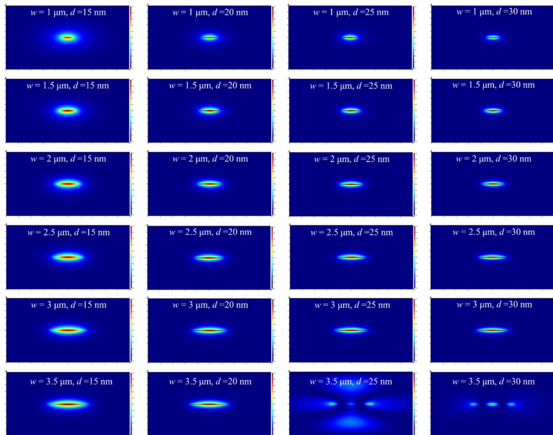
Figure 2. Electric field spatial distribution of Au stripe waveguide when the width w = 1, 1.5, 2, 2.5, 3, 3.5 \mu\text{m} and d = 15, 20, 25, 30 nm, respectively.
