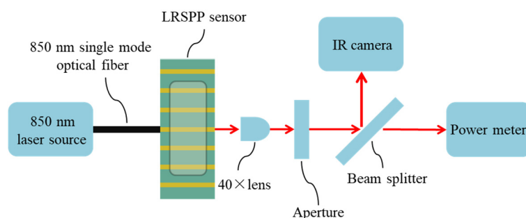
Figure 12. Schematic diagram of setup for characterizing LRSPP waveguide sensors.
