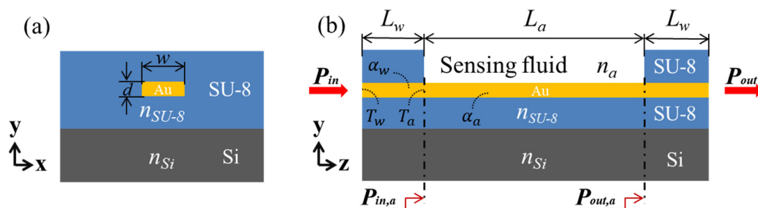
Figure 1. Schematic diagram of the straight long-range surface plasmon polariton (LRSPP) waveguide refractive index (RI) sensor: (a) Constructed by embedding the Au stripe of width w and thickness d in the polymer SU-8, and (b) with a microfluidic channel etched over the Au stripe to define the sensing region.
