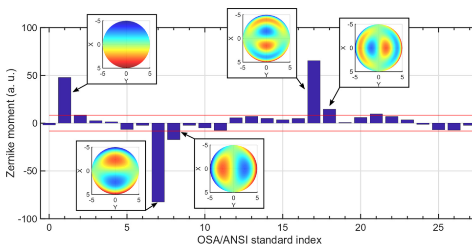
Figure A1. A Zernike decomposition of the operating deflection shape shown in Figure 3(C)c. The dominating mode carries index 7.
