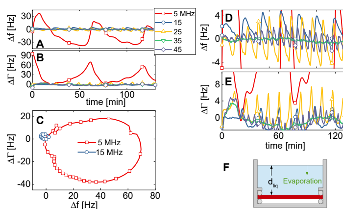
Figure 7. When mounting the resonator horizontally in an open cell (F) and letting the liquid evaporate, one observes coupled resonances (A–C). The vertical enlargement (D and E) shows the coupled resonances on the overtones. Because of the reduced wavelength, these are more densely spaced than the coupled resonances on the fundamental mode. Furthermore, and more importantly, they occur at a much-reduced amplitude.
