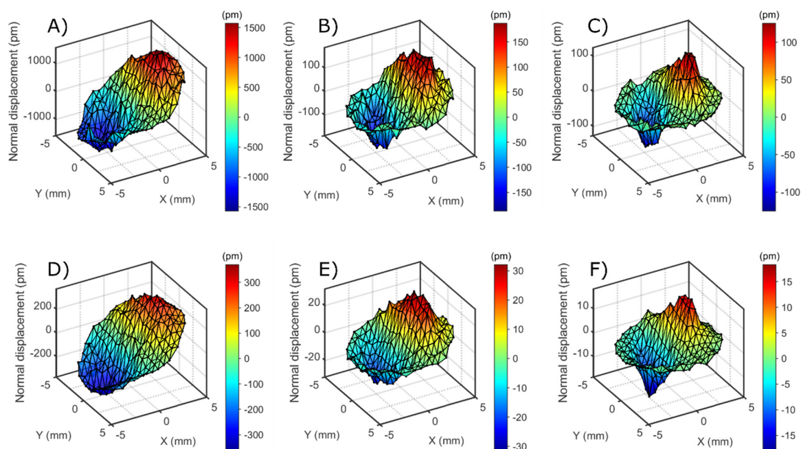
Figure 3. Operating deflection shape in normal direction (diameter of plate: 14 mm). (A)–(C): in air. (D)–(F): rear side in contact with water; Frequencies: (A),(D): 5 MHz, (B),(E): 15 MHz, (C),(F): 25 MHz.
