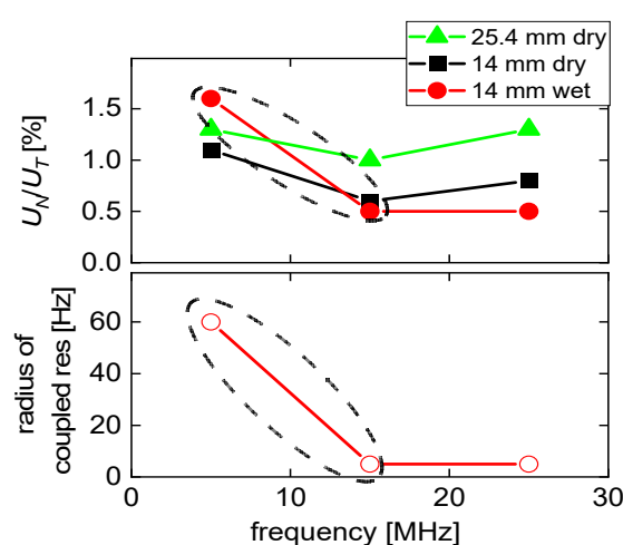
Figure 8. Results from Table 1 and Table 3 displayed in graphical form. U_N/U_T -ratios and the radius of the circle in the polar diagram (Figure 7(C)) both decrease when going from 5 MHz to 15 MHz.
