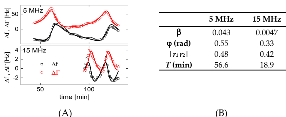
Figure 9. (A): Fits of Equation (11) to a subset of the data from Figure 7 (5 MHz and 15 MHz). The cuvette resonances are reproduced. (B) Corresponding fit parameters.
