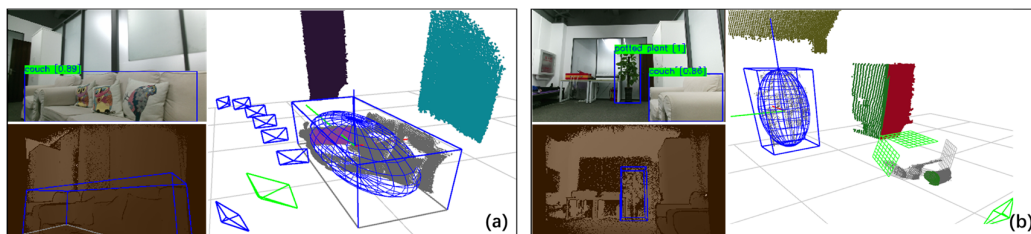
Figure 15. Complete and partial constraints of a mobile robot in the home-like environment. (a) a sofa with limited observation angle; (b) a sofa occluded by another one. Detailed description can be found in Figure 10.
