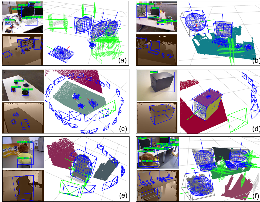
Figure 12. Complete and partial constraints of the TUM-RGB-D dataset. (a) fr1_desk; (b) fr2_desk; (c) fr2_dishes; (d) fr3_cabinet; (e) fr3_teddy; (f) fr3_long. Detail description can be found in Figure 10.
