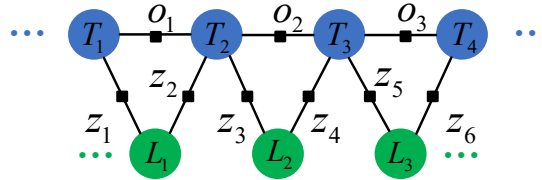
Figure 8. A factor graph for object simultaneous localization and mapping (SLAM). The node consists of the robot state \mathbf{T} and the object landmark \mathbf{L} expressed by the quadrics model. The edges are composed of camera-objects constraints \mathbf{z} and odometry constraints \mathbf{o} .
