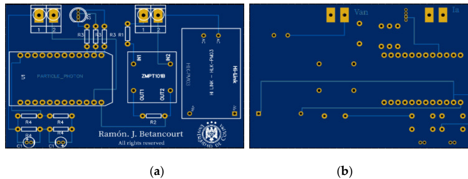
Figure 7. PCB board of the proposed meter system: (a) Top view, (b) Bottom view.
