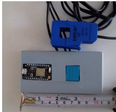
Figure 8. Photography of the IoTBEMS.
