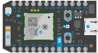
Figure 4. Physical structure of the Photon Particle®.
