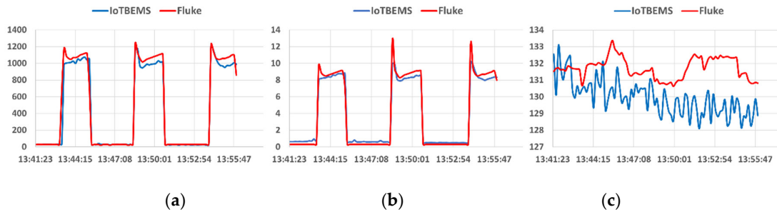
Figure 9. Comparison with Fluke 435 II: (a) Watts, (b) Amperes, (c) Volts.
