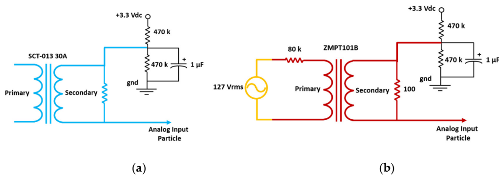
Figure 6. Coupling circuits based on instrument transformers: (a) Coupling circuit for current sensor, (b) Coupling circuit for voltage sensor.
