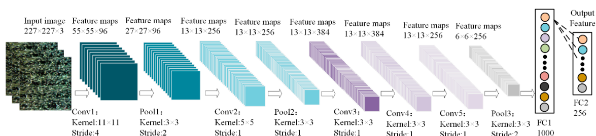
Figure 3. Convolutional neural network structure. Kernel represents the size of the convolution kernel (pixels), Stride represents the sliding step size, Conv1, Conv2, Conv3, Conv4, Conv5 represent the first, second, third, fourth, and fifth convolutional layers, and Pool1, Pool2, and Pool3 represent the first, second, and third pooling layer, FC1 and FC2 represent fully connected layer.
