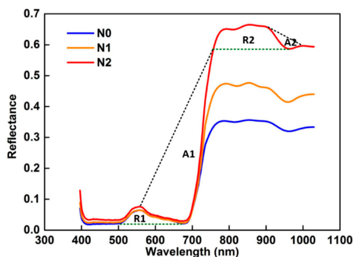
Figure 2. Characteristic absorption and reflection positions of the winter wheat for the three nitrogen treatments. (A) Absorption position, and (R) reflection position.
