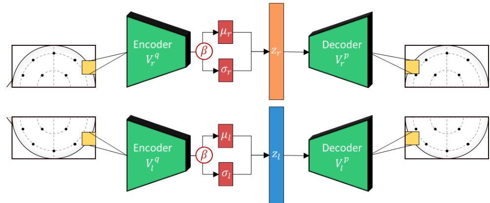
Figure 4. The lateralized beta-VAE implementation used in this work. Each hemisphere is composed of an encoder and decoder pair with the encoder generating a stochastically sampled embedding, z , based on outputs, \mu and \sigma . Separate weights are used to encode the features for each of the hemispheres to adhere to neuroscience theories of lateralization.
