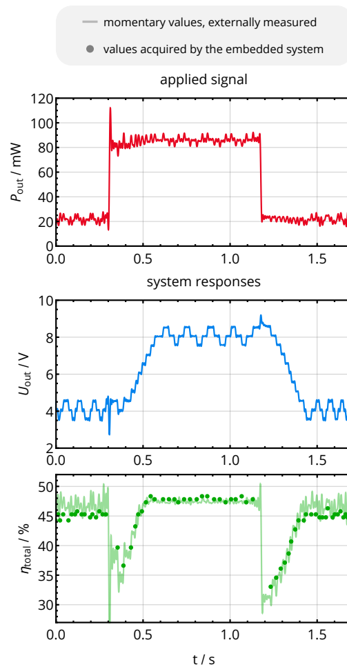
Figure 15. Reaction of the complete power feedback and maximum efficiency point tracking system with respect to a transient change in power consumption P_{out} for a coil separation distance of d_{12} = 10 mm ( M_{12} = 46 nH). The output voltage shows the characteristic behavior of the perturb-and-observe algorithm, oscillating around the optimal voltage for a constant output power level. Upon a load change, the system reestablishes the maximum efficiency level.
