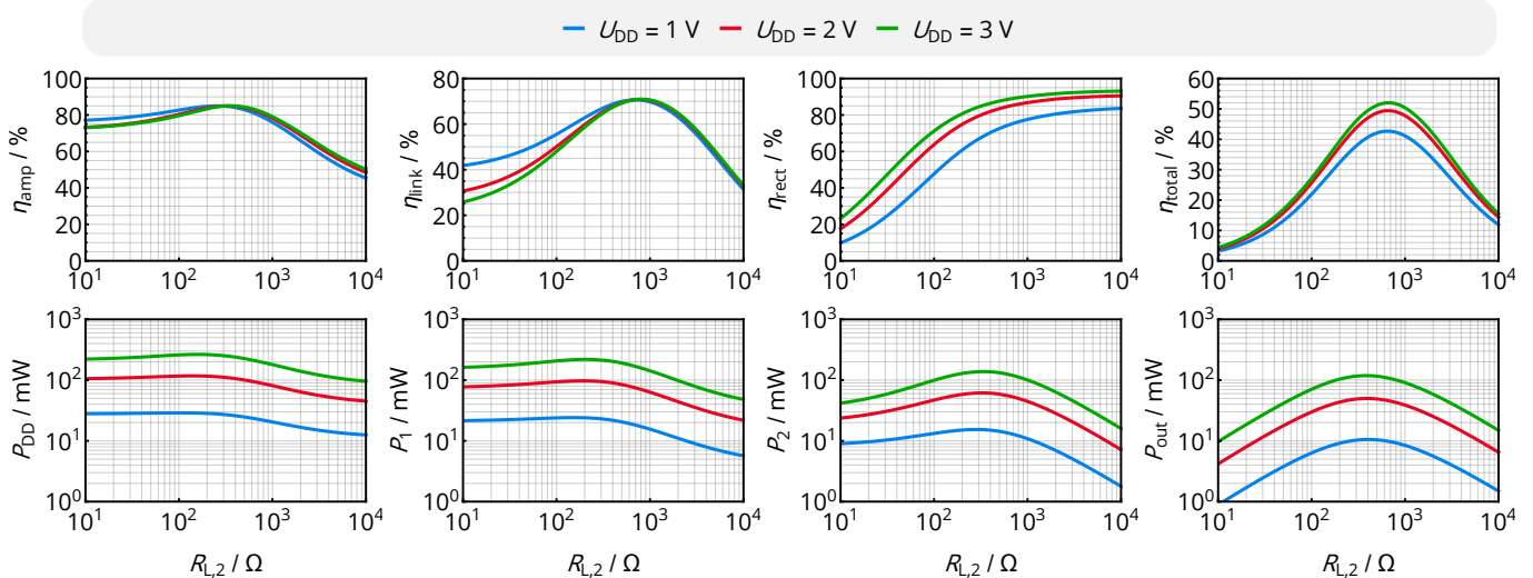
Figure 5. Power and efficiency levels of the main components of the WPT interface versus the DC load resistance R_{L,2} . All components' efficiency levels scale differently with load resistance and different overall power levels determined by U_{\text{DD}} . The overall efficiency \eta_{\text{total}} is still optimized by a dedicated DC load resistance R_{L,2} .
