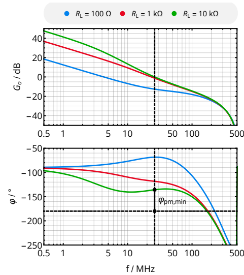
Figure 8. Bode plot of the open-loop transfer function G_o[e^{j2\pi f_0}] for M_{12} = 10 nH, the control parameters (K_P, T_I, T_D) = (0.7, 0.01 s, 0 s) and different DC load resistances R_{L,2} , resulting in the minimal phase margin of 44^\circ for R_{L,2} = 10 kΩ.
