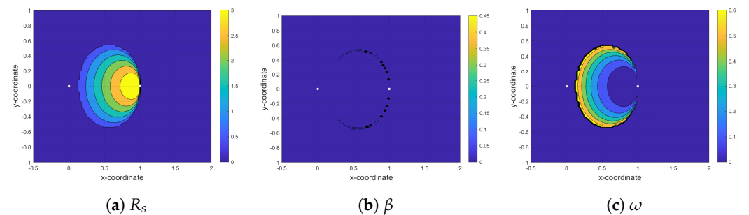
Figure 6. Maximizing rate at the second receiver (SR) by finding the optimum value for time fraction ( \beta ) and power fraction ( \omega ) in the AF-NOMA protocol.
