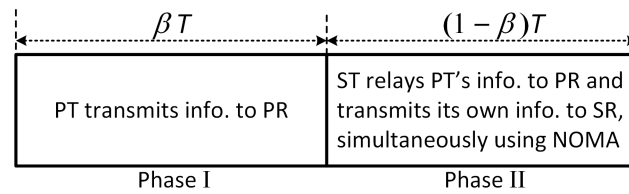
Figure 2. Time block of cooperative NOMA.
