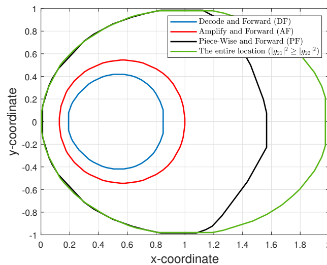
Figure 8. A comparison of the locations that PF-NOMA, DF-NOMA and AF-NOMA can cover for the rate greater than or equal to 0.5 bit/s/Hz at the second receiver (SR).
